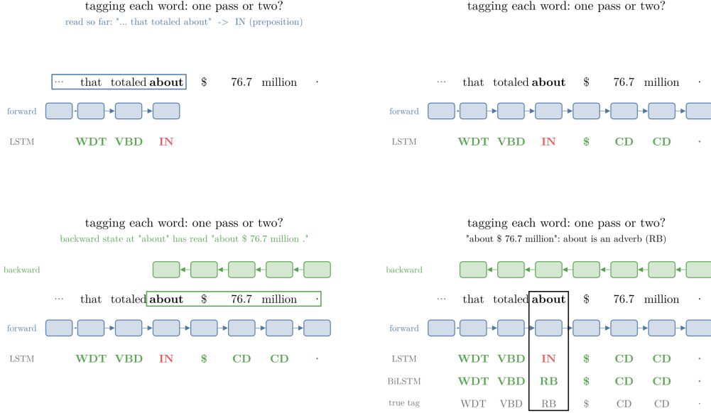
Figure 2: Tagging a real CoNLL-2000 test sentence. The forward pass (blue) sweeps left to right and the unidirectional LSTM gives its tags (red: wrong). The backward pass (green) then sweeps right to left from the last word. Joining both states, the BiLSTM tags “about” RB, the true tag, because it has read “$ 76.7 million”. Tags from the Notebook’s LSTM (64 nodes) and BiLSTM, seed 1
