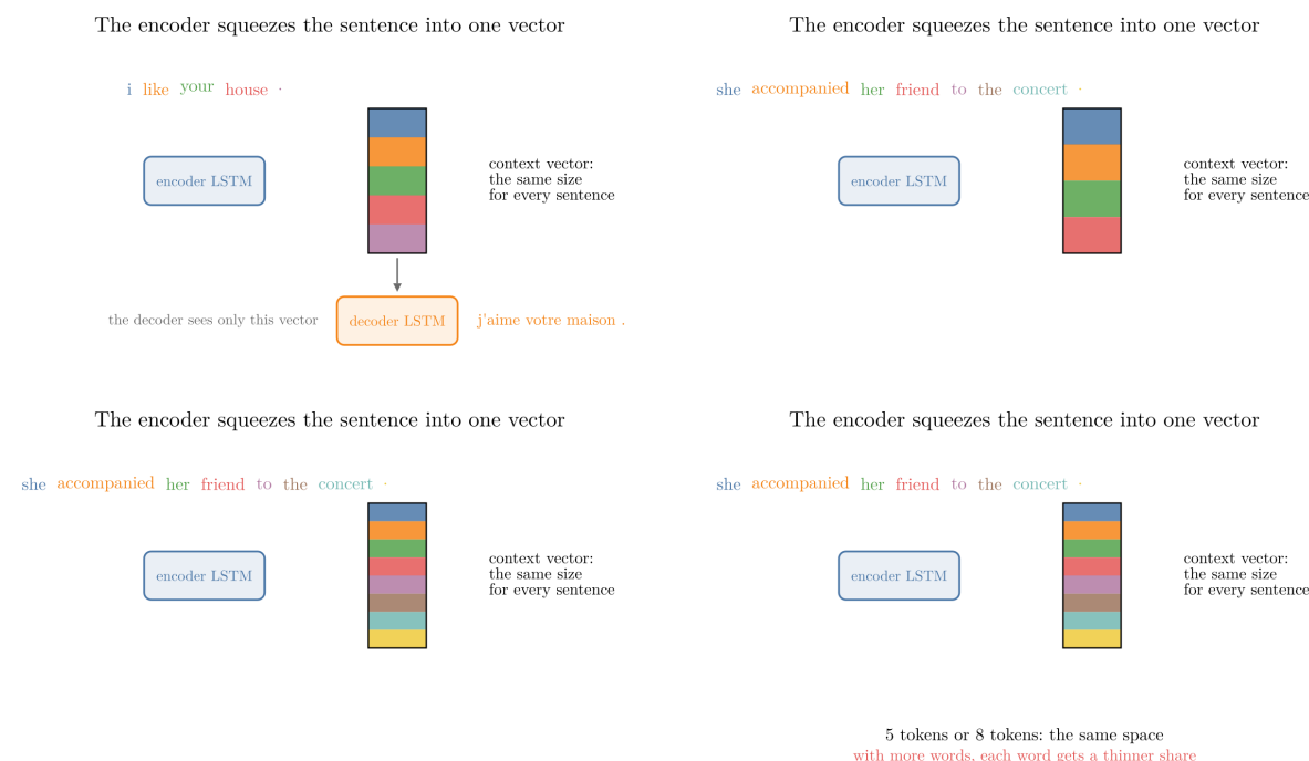
Figure 2: The encoder reads one word per step and ends with one context vector of fixed size, the decoder’s only view of the input. A 5-token sentence and an 8-token sentence end in the same space, so each word gets a thinner share. A picture of the idea, not of the LSTM’s actual numbers
