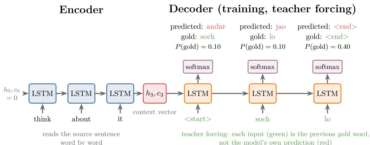
Figure 3: Training on one observation. The decoder’s input at each step (green) is the previous gold word, not the model’s own prediction (red)
