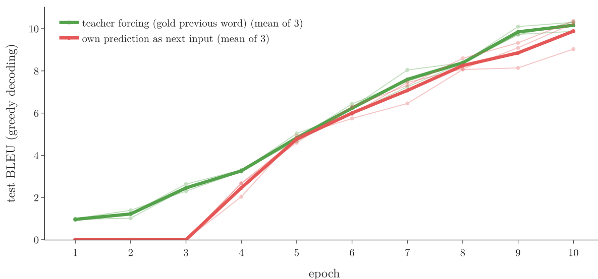
Figure 4: Test BLEU after each epoch. Thin lines: 3 runs each; thick lines: their mean. With teacher forcing (green) the model starts scoring at once; trained on its own predictions (red) it scores 0 for 3 epochs
