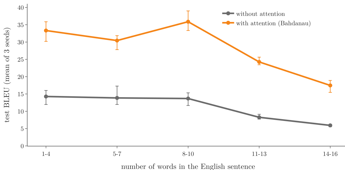
Figure 4: Test BLEU by English sentence length, mean of 3 runs, with the lowest and highest run as bars
