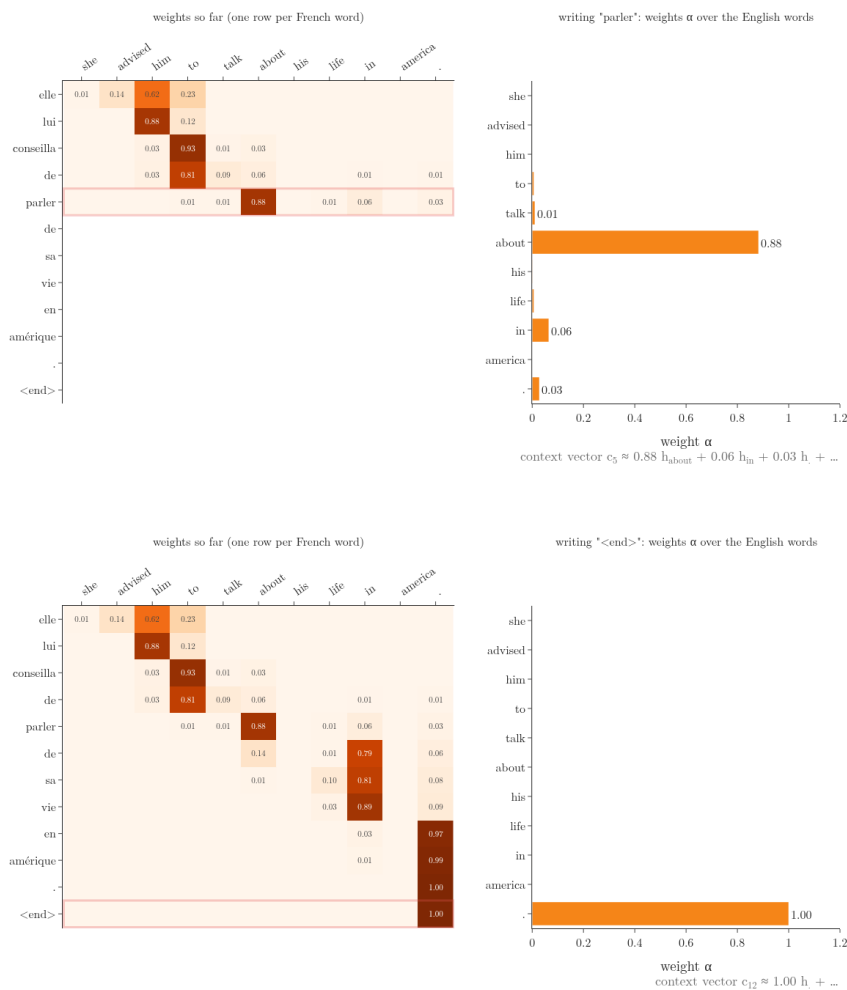
Figure 2: The trained attention model writing one French word per frame. Left: the weight grid filling row by row (current row outlined in red). Right: the current word’s weights over the English words, and the context vector they build
