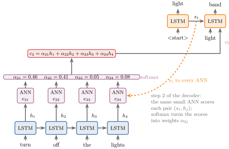
Figure 3: One decoder step with attention. The same small network scores every pair (s_1, h_j) ; softmax turns the scores into weights; the weighted sum c_2 joins the decoder’s input
