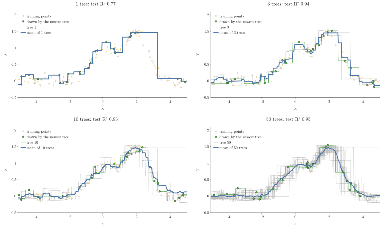
Figure 2: The bagging regressor built one tree at a time: every tree so far (grey), the newest tree and its 25 drawn points (green), and the mean of the trees, the bagging prediction (blue)
