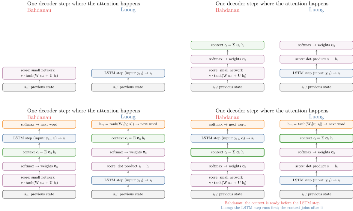
Figure 2: One decoder step in the two designs, built up one operation at a time from the bottom. Bahdanau scores the previous state and computes the context before the LSTM step; Luong runs the LSTM step first, scores the new state by a dot product, and joins the context after the step
