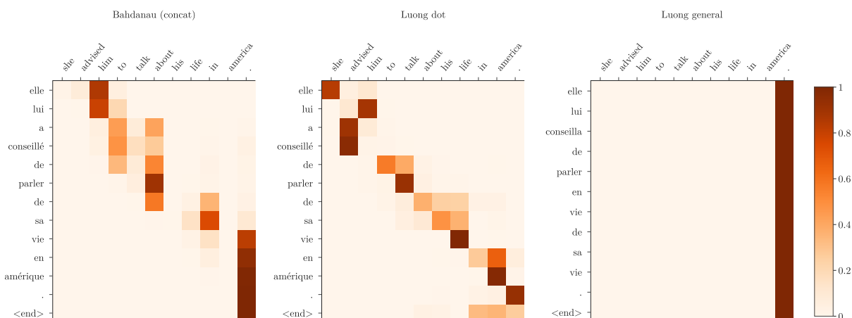
Figure 3: Attention weights of the three trained models on the same real test sentence. Bahdanau and Luong dot both translate it exactly; Luong general puts all its weight on the final full stop
