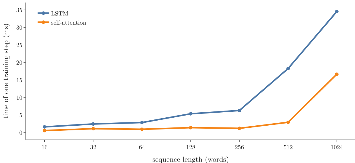
Figure 3: Time of one training step against sequence length (log scale). The LSTM’s time grows from the start; self-attention stays flat up to 256 words
