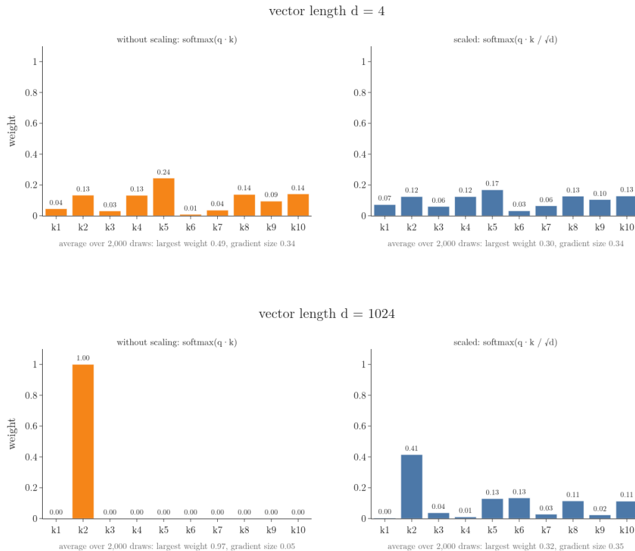
Figure 4: One random query against 10 random keys, using the first d numbers of each, for d from 1 to 1,024. Left: the softmax of the raw dot products collapses onto one key. Right: divided by \sqrt{d} , the weights stay spread out. Under each panel, the Notebook’s averages over 2,000 draws
