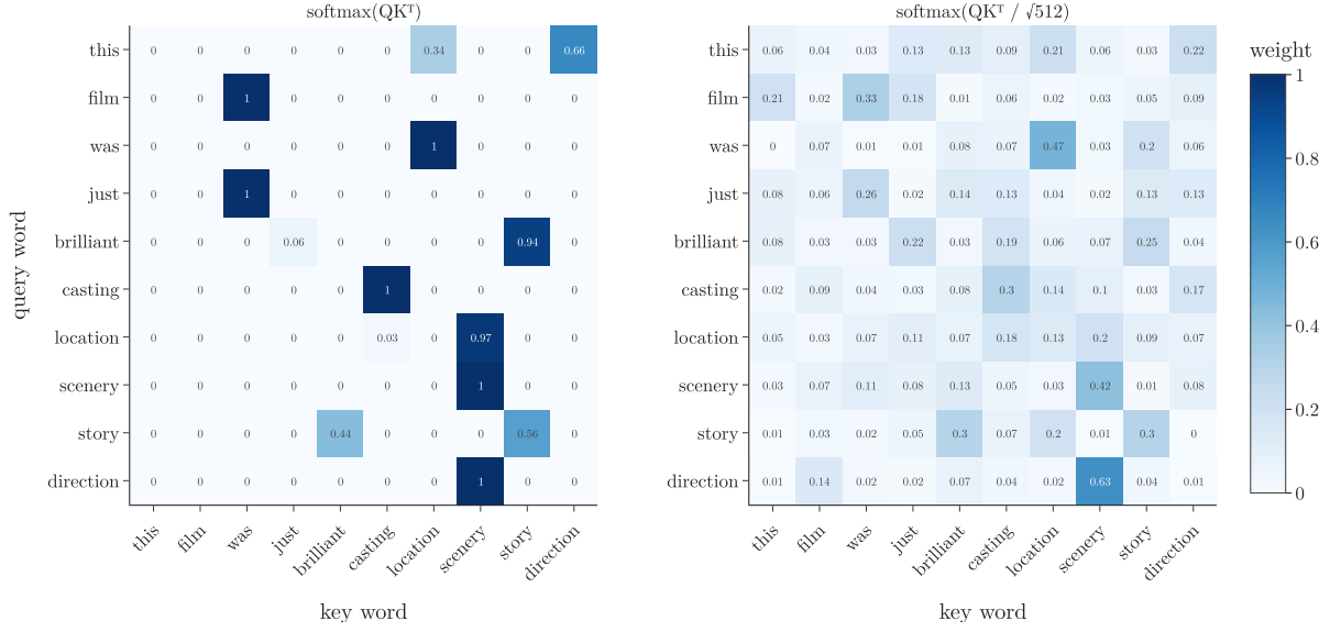
Figure 5: Attention weights for “this film was just brilliant casting location scenery story direction”, d_k = 512 , untrained random weights. Left: without scaling, most rows are a single 1. Right: divided by \sqrt{512} , the weights are spread out
