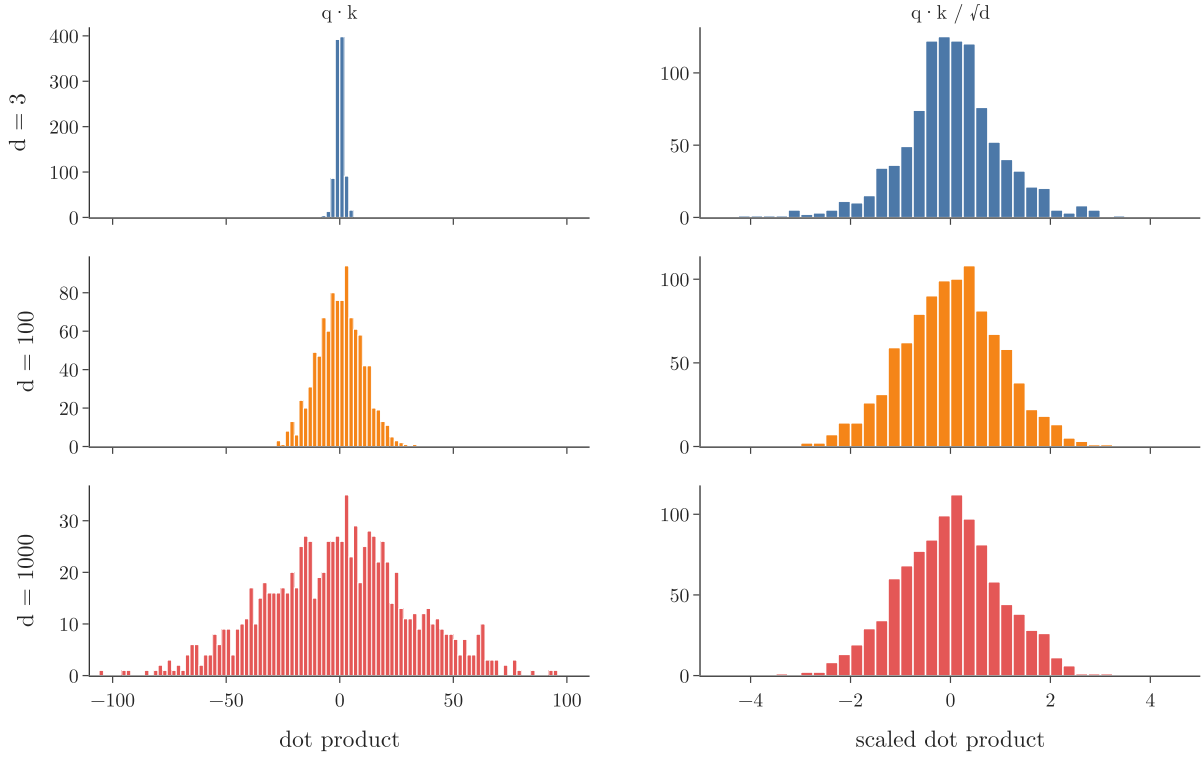
Figure 2: Histograms of 1,000 dot products each, one row per vector length d (each row has its own count scale). Left: the spread grows with d . Right: after dividing by \sqrt{d} , the three histograms have the same spread
