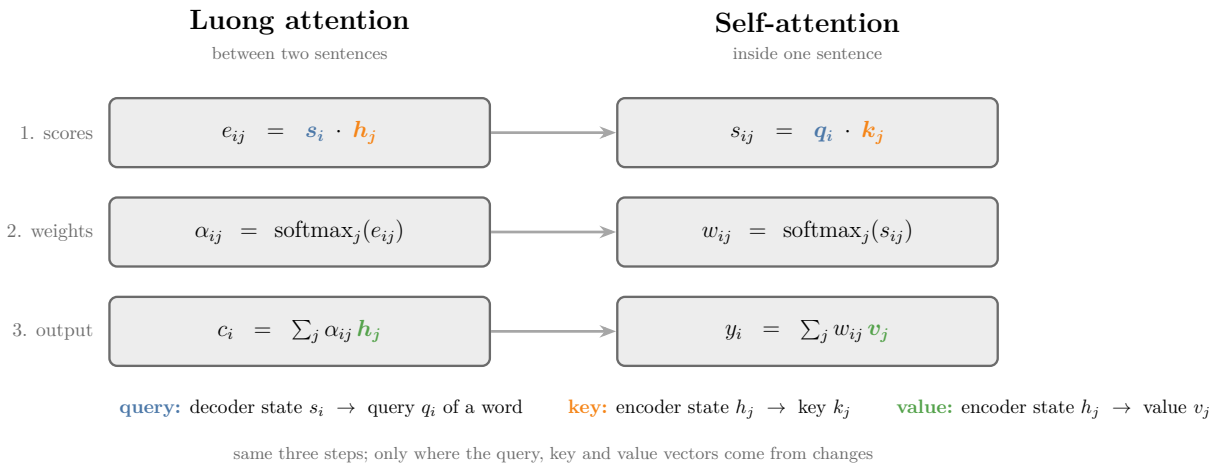
Figure 2: The three equations of Luong attention (left) and of self-attention (right), step by step. The colours mark the only substitutions: the decoder state becomes a query (blue), the encoder state used for comparing becomes a key (orange), and the encoder state that is mixed becomes a value (green)
