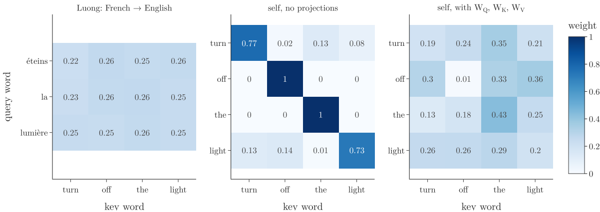
Figure 3: Weight matrices from the Notebook (untrained networks, so the values have no meaning yet; the shapes do). Left: Luong attention, French queries over English keys, 3 \times 4 . Middle: self-attention on the English embeddings without projections. Right: with W_Q , W_K , W_V and scaling. Both self-attention matrices are 4 \times 4
