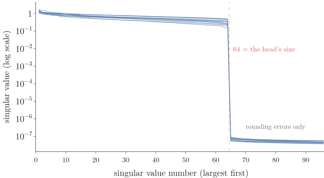
Figure 3: BERT-base, layer 1: the singular values of each of the 12 heads’ value maps W_V^i W_O^i , largest first (log scale). All 12 drop to rounding-error size after exactly 64
