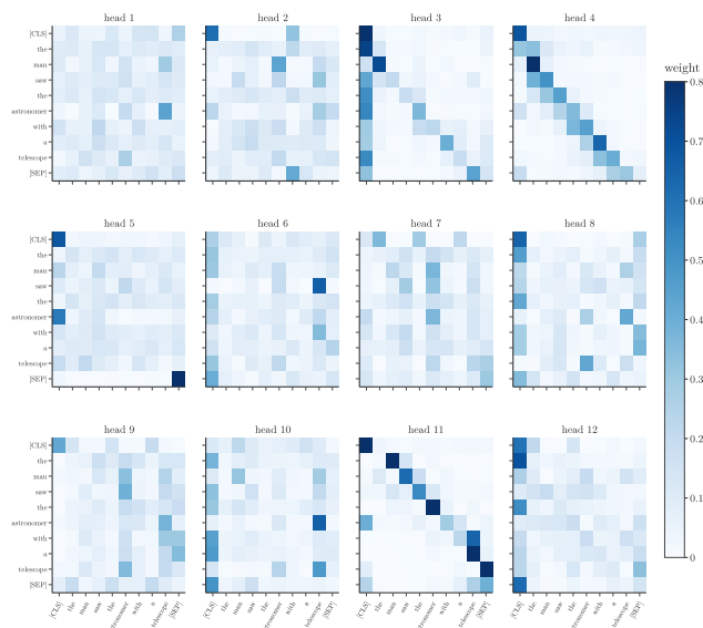
Figure 5: The 12 heads of BERT-base’s first layer on the same sentence (rows: query word, columns: key word)
