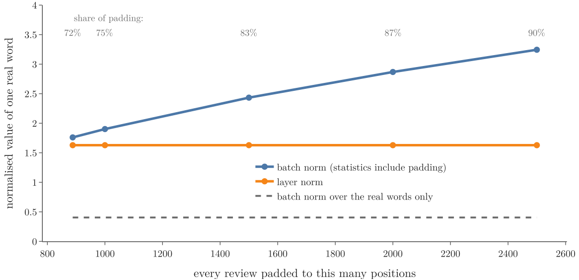
Figure 3: The same real word after normalisation, as the batch is padded to more positions. Batch normalisation (blue) drifts with the amount of padding, and is far from batch normalisation over the real words alone (dashed, 0.40). Layer normalisation (orange) does not change
