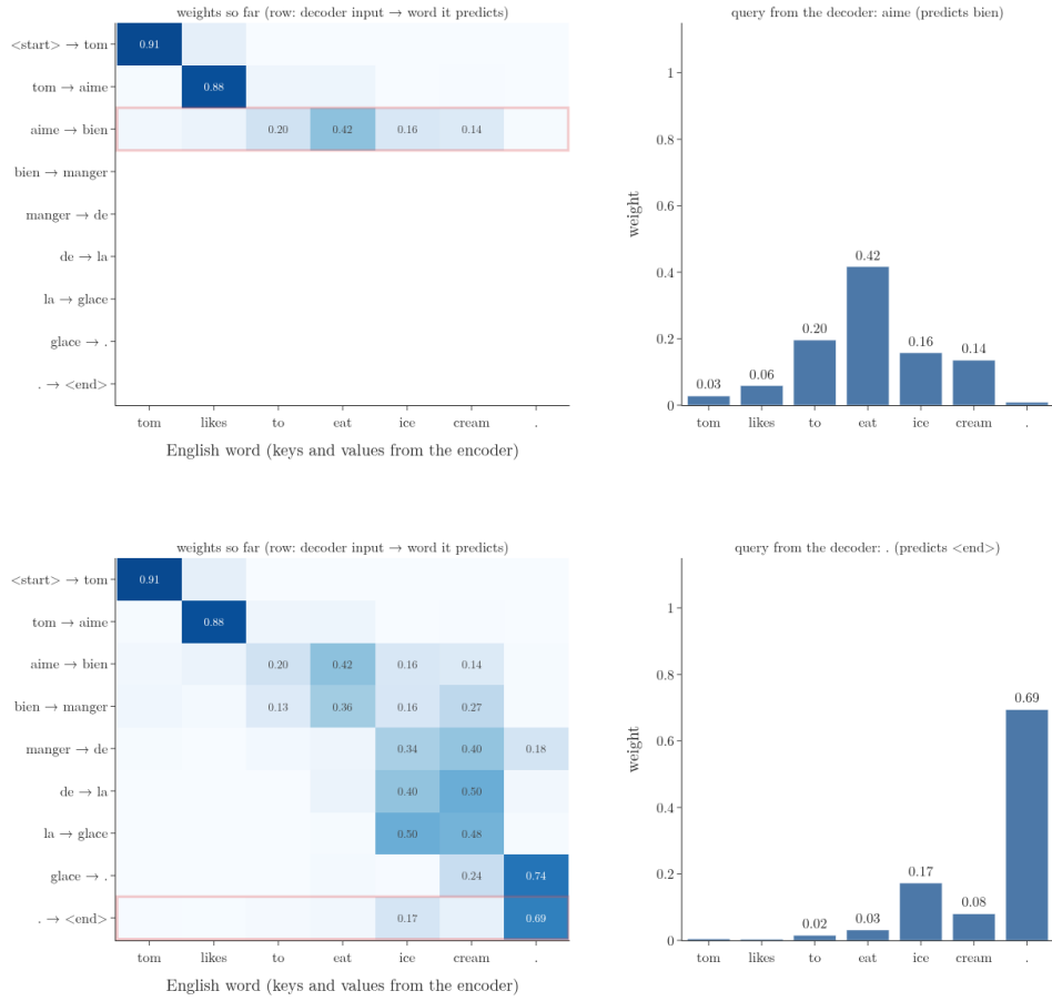
Figure 2: Cross-attention of the trained model of section 7 on “Tom likes to eat ice cream.”, one French position per frame. Left: the 9 \times 7 weight grid filling row by row. Right: the current query’s weights over the English words, whose keys and values come from the encoder
