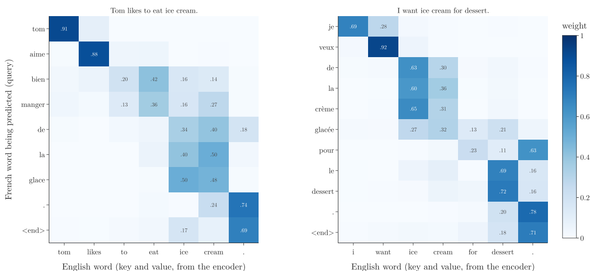
Figure 3: Cross-attention weights of the trained model on two sentence pairs it never saw. Rows: the French word being predicted; columns: the English words. Weights below 0.1 are not written
