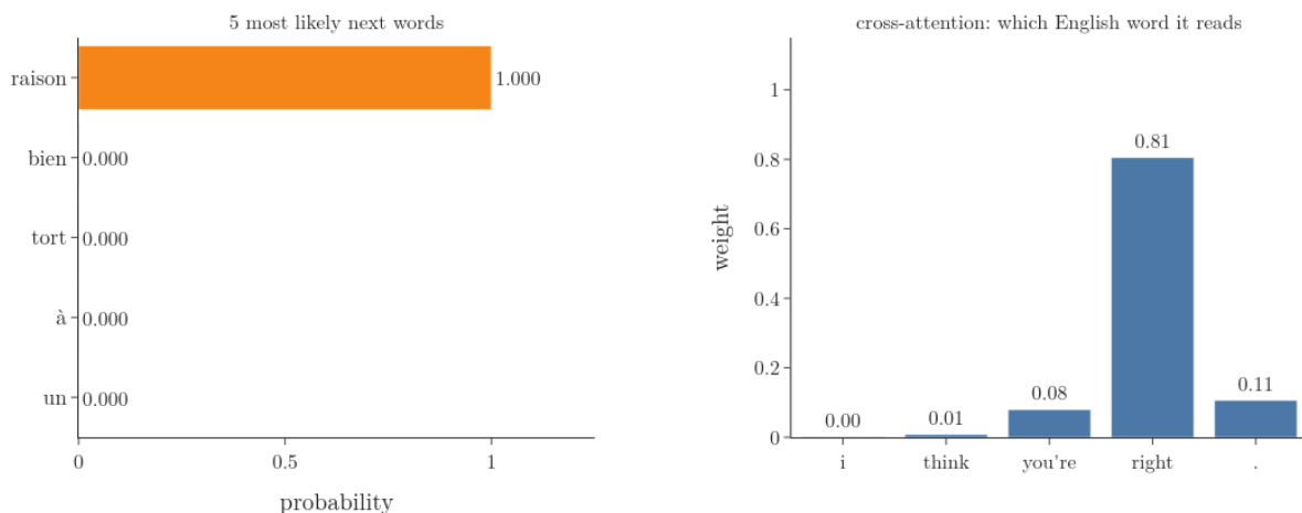
Figure 4: The trained transformer translating “i think you’re right .” one step per frame. Left: the 5 most likely next words (the chosen one in orange). Right: the cross-attention weights, in the last decoder block, of the position that predicts the next word (mean of 4 heads)
