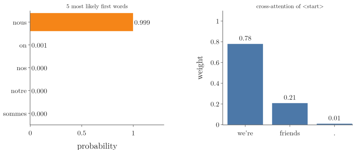
Figure 3: Step 1 of translating “we’re friends .”: the 5 most likely first words, and the cross-attention weights of <start> on the English words (last decoder block, mean of 4 heads)
