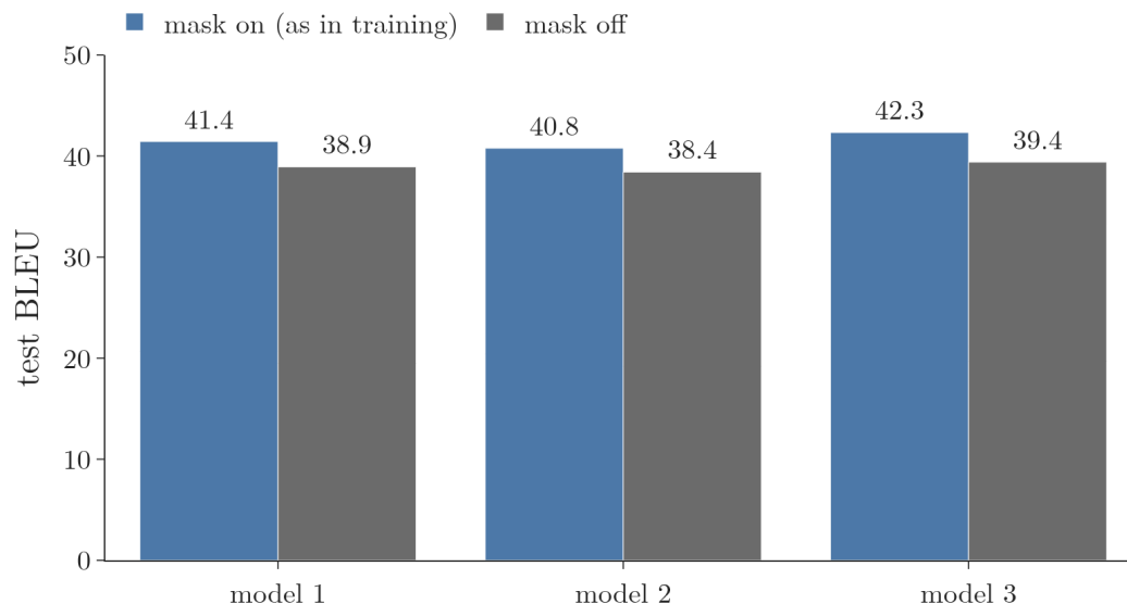
Figure 5: Test BLEU of 3 trained models with the mask on at inference (as in training) and switched off
