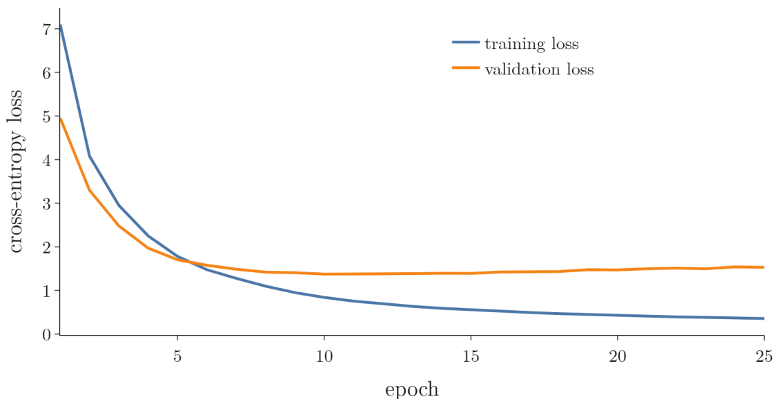
Figure 2: Training the small transformer: the cross-entropy loss on the training pairs and on the 5 percent held out for validation, per epoch
