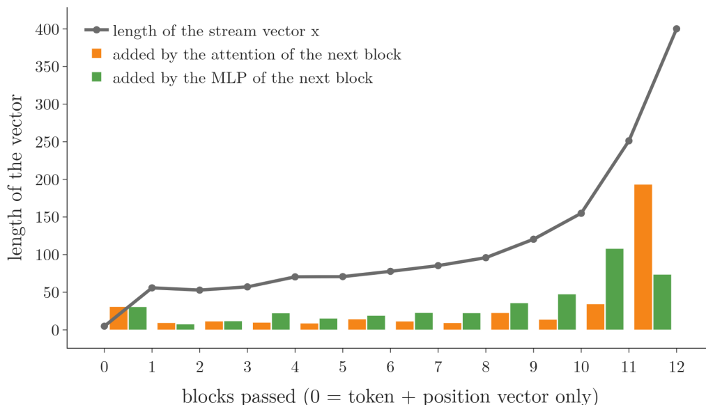
Figure 3: Length of the stream vector of " of" after each block of GPT-2 small (grey), and the lengths of the vectors added by each block's attention (orange) and MLP (green)
