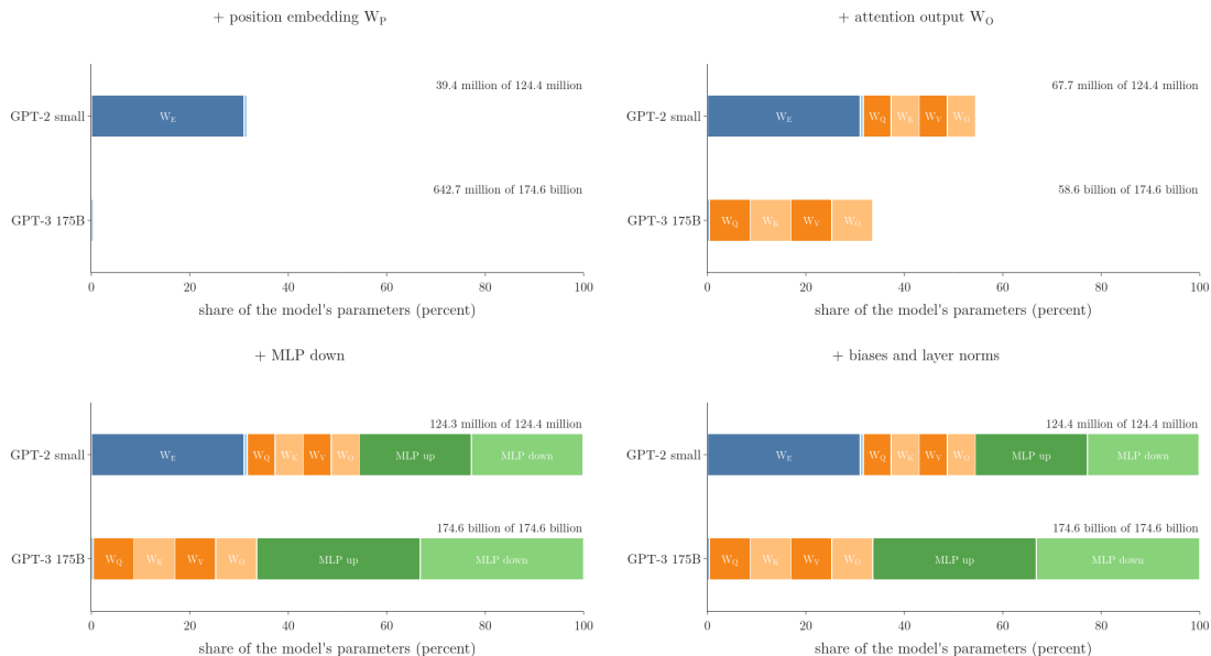
Figure 5: Running tally of parameters, one kind of matrix at a time, as a share of each model. Blue: embeddings. Orange: attention ( W_Q, W_K, W_V, W_O ). Green: MLP. Grey (thin): biases and LayerNorms
