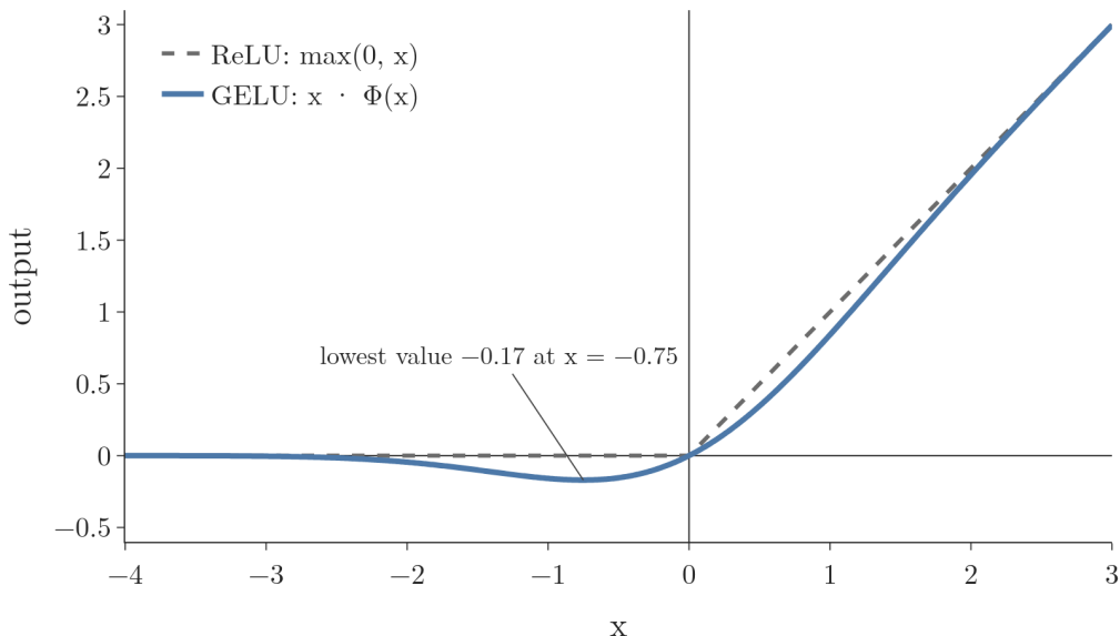
Figure 4: GELU and ReLU. For large positive x both give x ; for large negative x both give about 0; near 0 GELU is a smooth curve that dips to -0.17
