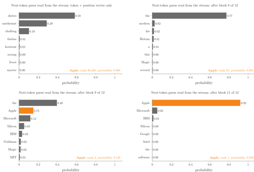
Figure 3: Logit lens on GPT-2 small, “Steve Jobs was the founder of”: the 8 most likely next tokens read from the last token’s stream after each block. Orange: ” Apple”
