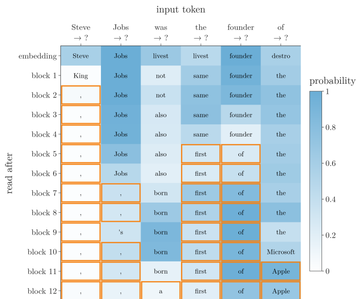
Figure 4: Logit lens grid (after nostalgebraist 2020): the top guess at every position (columns) after every block (rows). Shade: its probability. Orange outline: the guess already equals the final one
