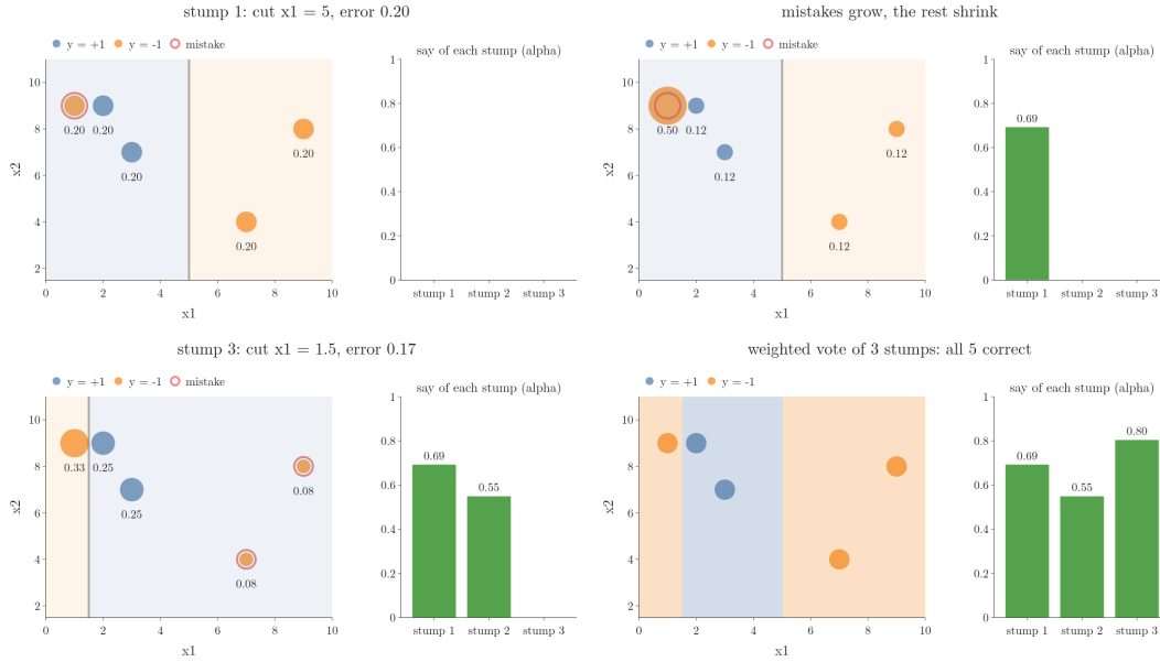
Figure 4: Three AdaBoost stages on the toy data. Dot size and label: the observation's weight. Line and shading: the stump's cut and the class on each side; red rings: its mistakes. Right: each stump's alpha. Last frame: the sign of the weighted vote.
