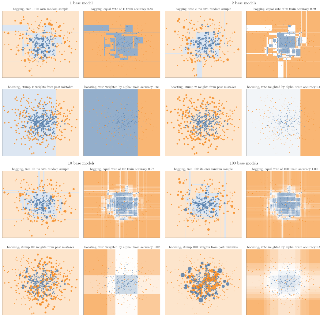
Figure 2: Bagging (top: fully grown trees, each on its own random sample; marker size = copies drawn) against AdaBoost (bottom: stumps; marker size = weight from earlier mistakes) on the noisy circles, one base model per frame. Right: the vote so far; white means a split vote
