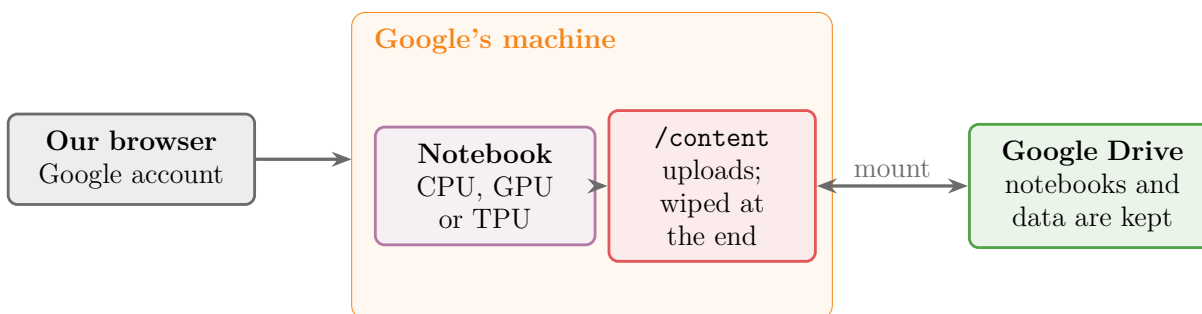
Figure 7: A Colab session: the notebook runs on Google's machine; only Google Drive outlives the session
