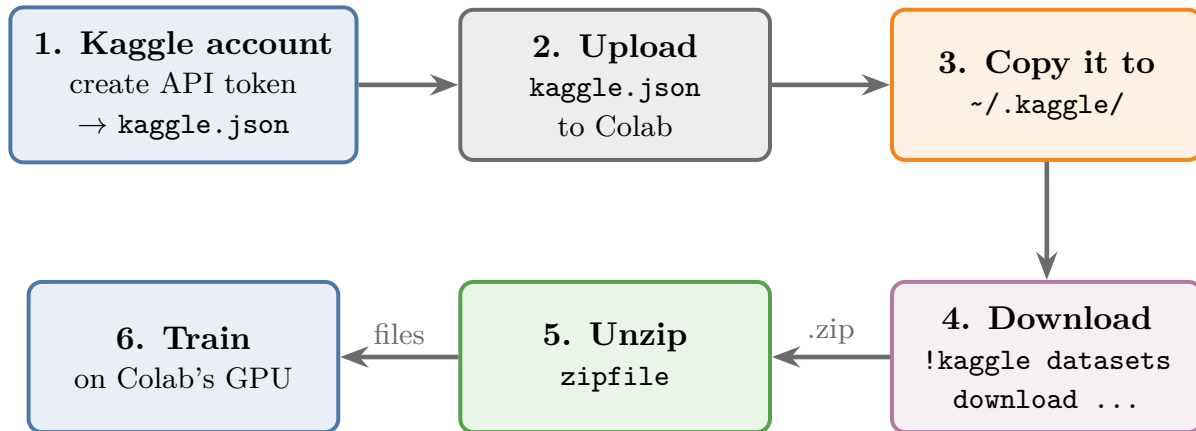
Figure 8: Downloading a Kaggle dataset straight into Colab
