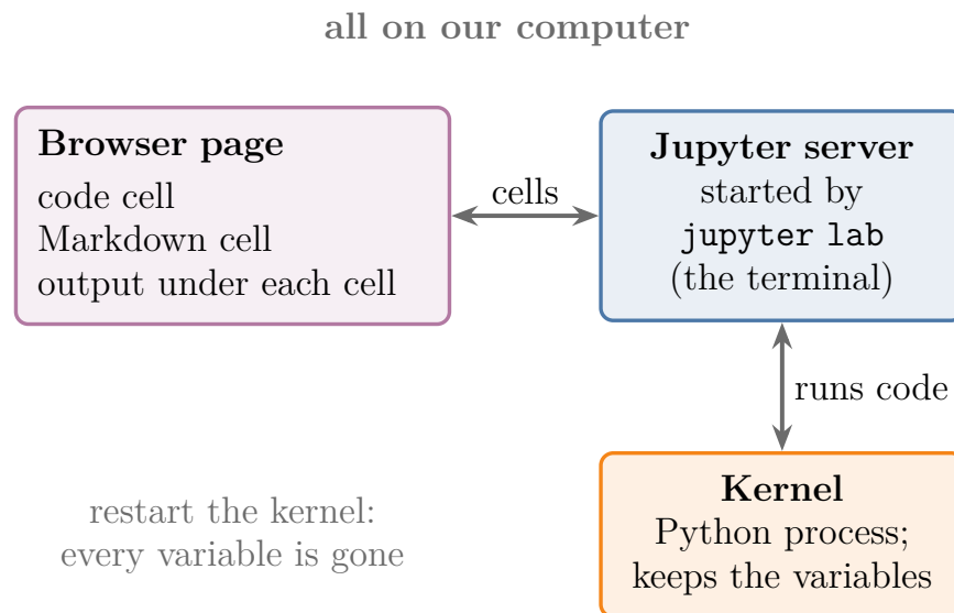
Figure 3: The three parts of local Jupyter: the browser page, the server in the terminal, and the kernel
