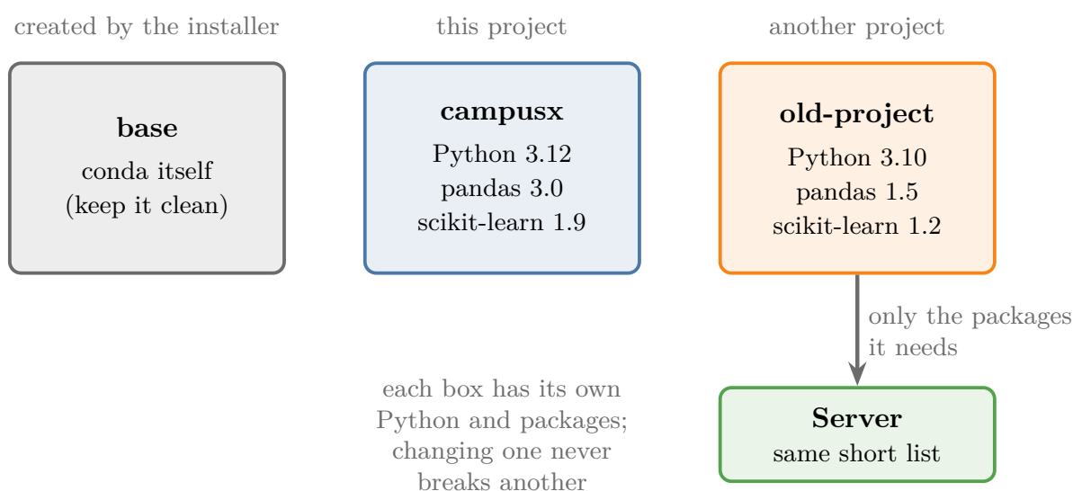
Figure 4: Separate environments, each with its own Python and packages
