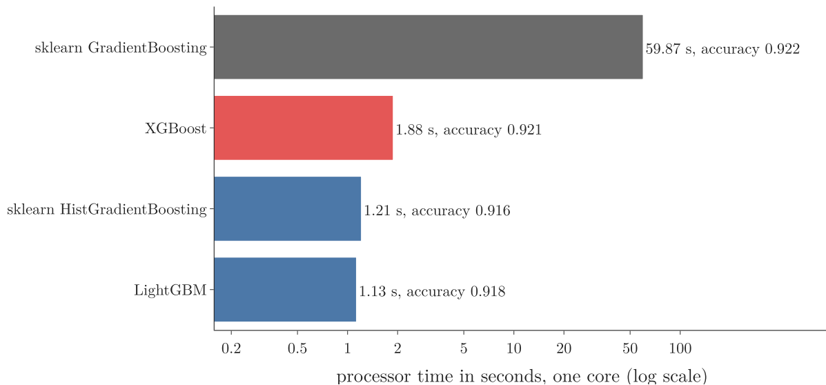
Figure 2: Processor time on 10,000 observations and 200 features, 100 trees of depth 3 in every library, one core each (log scale)
