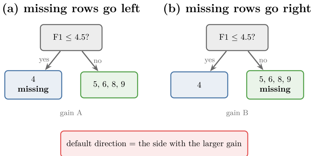
Figure 4: Sparsity-aware split finding: observations with a missing value are tried on each side; the side with the larger gain becomes the default direction
