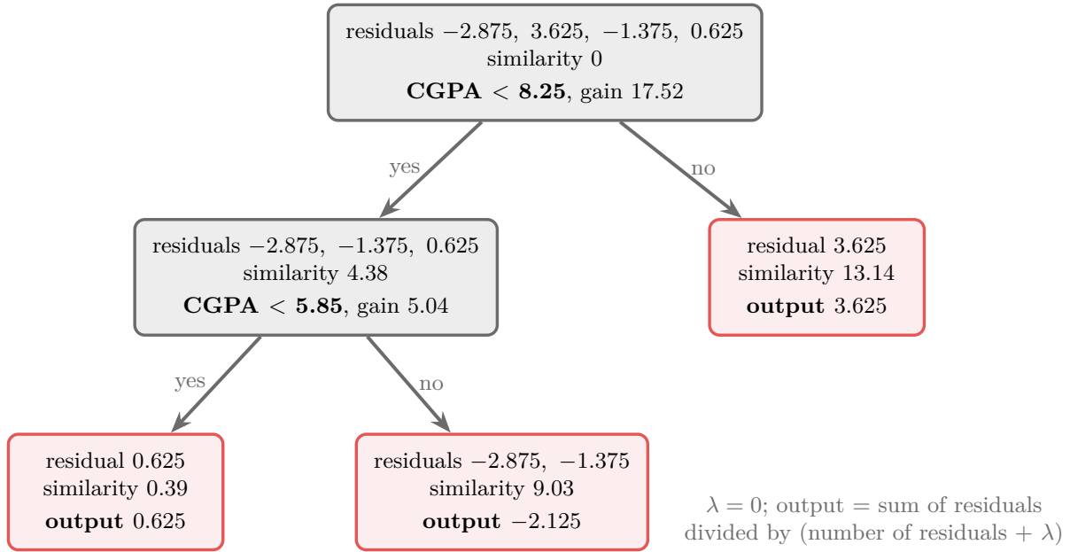
Figure 5: The first XGBoost tree: residuals, similarity scores, gains of the two splits and the outputs of the three leaves
