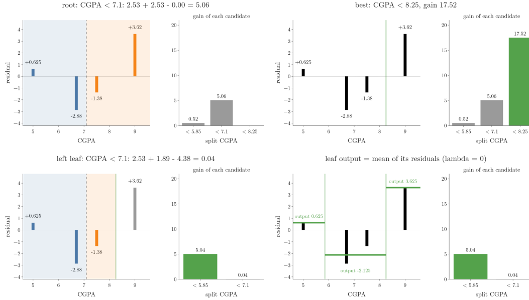
Figure 4: The XGBoost split search on the four students (lambda = 0). Left: the residuals, the sliding threshold and the locked splits (green). Right: the gain of each candidate, S_{\text{left}} + S_{\text{right}} - S_{\text{parent}} . Last frame: the outputs of the three leaves. The sliding-threshold picture follows StatQuest’s “XGBoost Part 1: Regression” (Starmer)
