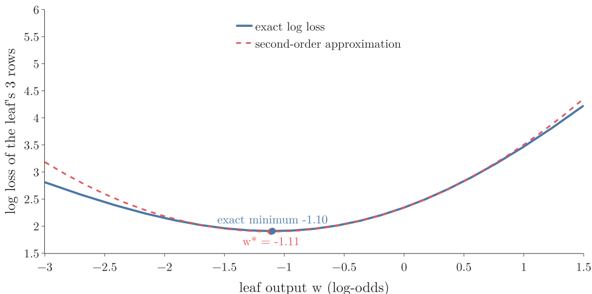
Figure 5: Exact log loss of this leaf’s three observations (blue) and its second-order approximation (red) as the leaf output w changes: they agree near 0, and their minima are close
