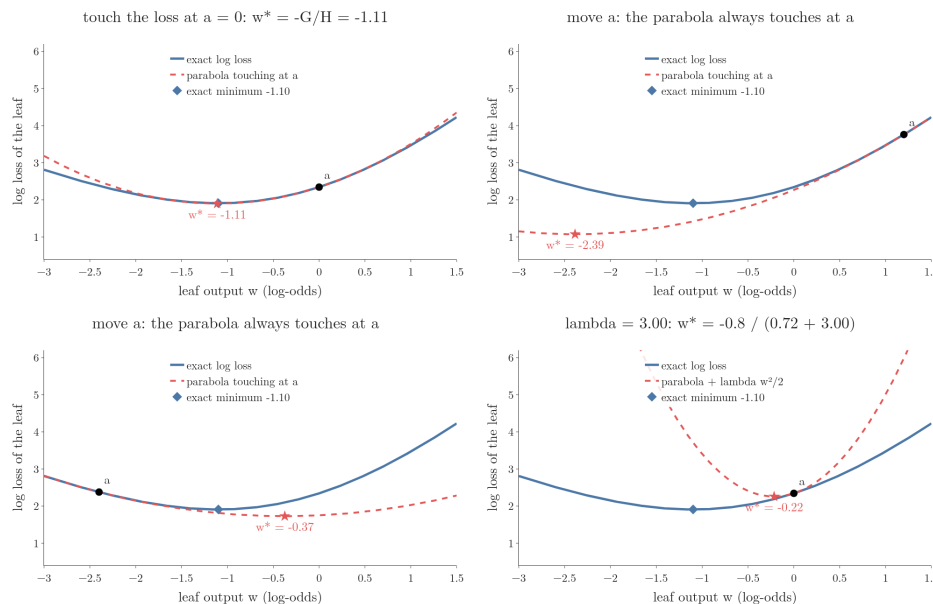
Figure 6: The second-order approximation of this leaf’s log loss, animated. The red parabola touches the exact loss (blue) at the expansion point a ; the star is its minimum, the Newton step. Last part: back at a = 0 , \lambda grows and the leaf output w^* shrinks towards 0. Watching the minimum move towards 0 as \lambda grows follows StatQuest’s “XGBoost Part 3 (of 4): Mathematical Details” (Starmer)
