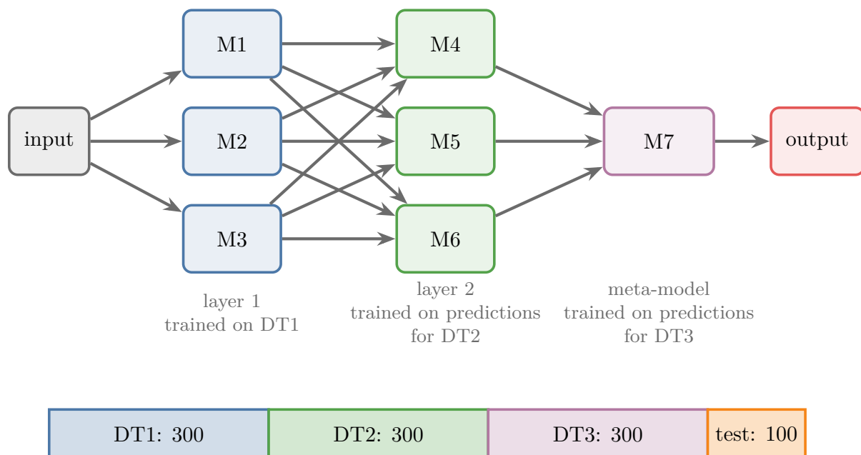
Figure 4: Two layers of base models and a meta-model, trained with blending on three hold-out sets of 300 observations
