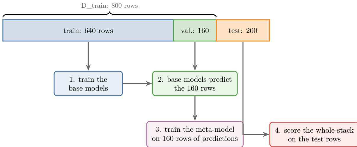
Figure 2: Blending: 1,000 observations split into 800 for training and 200 for testing; the 800 are split again into 640 for the base models and 160 for the meta-model
