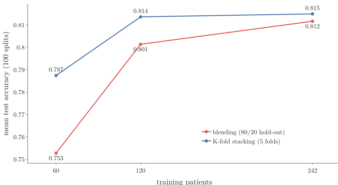
Figure 6: Mean test accuracy of blending and K-fold stacking on the heart data, for 60, 120 and 242 training patients, averaged over 100 random splits
