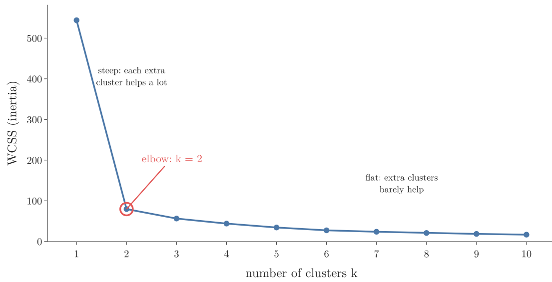
Figure 3: Elbow curve: WCSS against k for the 272 Old Faithful eruptions (standardized); the curve bends at k = 2
