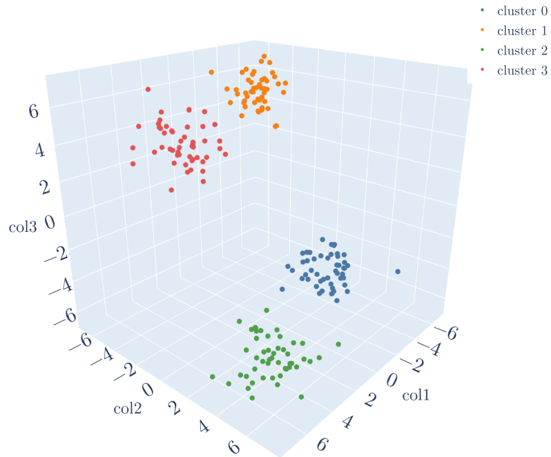
Figure 3: k-means with k = 4 on 200 points with three features
