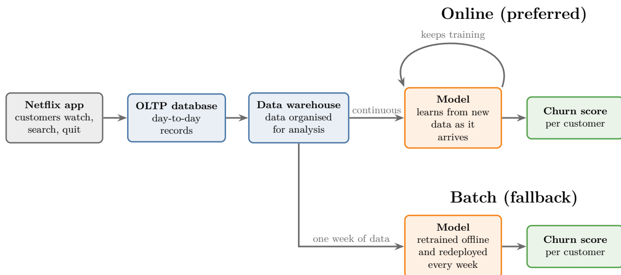
Figure 10: Online learning for churn, with batch learning as a fallback
