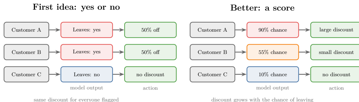
Figure 6: A yes or no answer gives everyone the same discount; a score lets the discount grow with the risk
