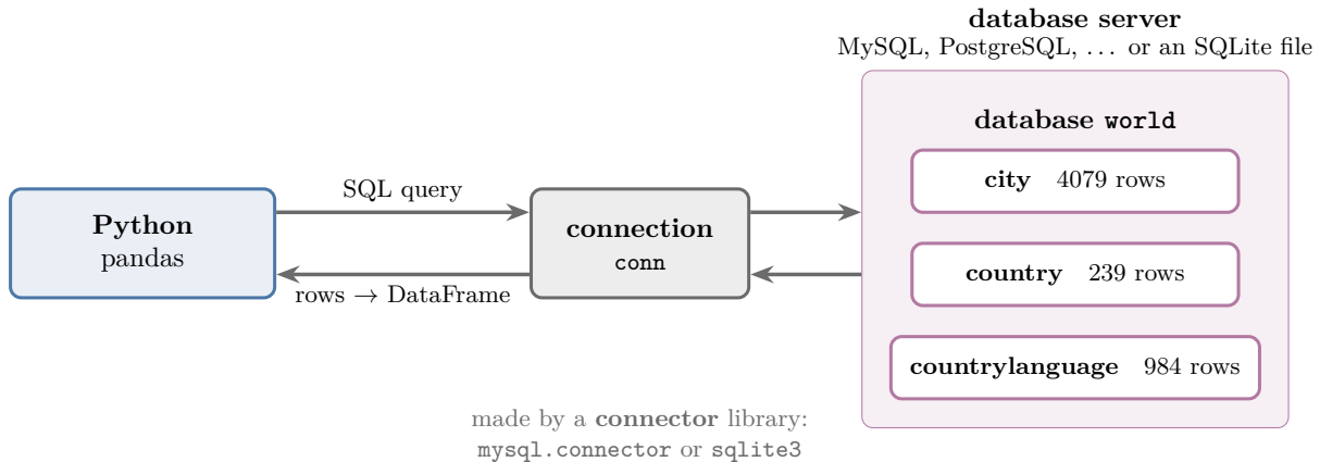
Figure 5: Python talks to the database through a connection
