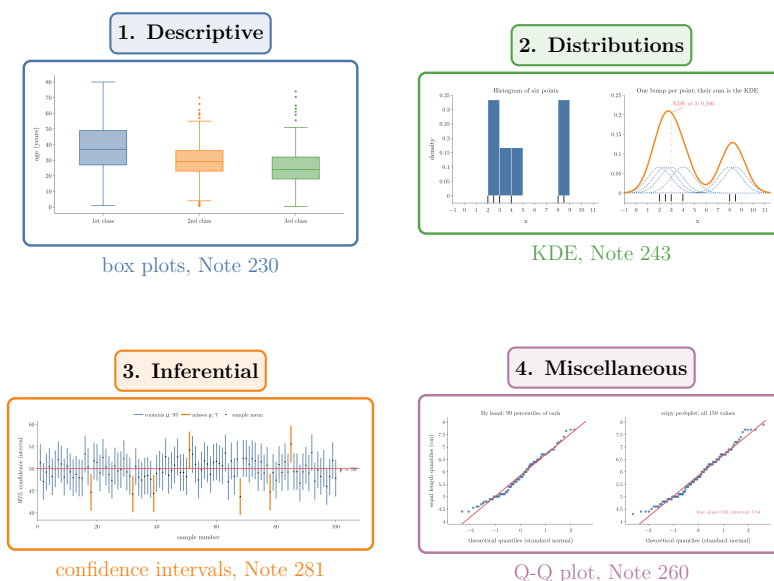
Figure 2: One key figure from each module: box plots of Titanic ages (Note 230), a kernel density estimate built from bumps (Note 243), 100 confidence intervals (Note 281) and a Q-Q plot of iris sepal lengths (Note 260)
