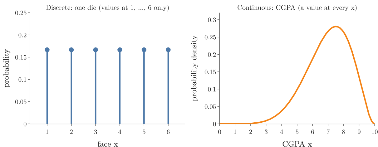
Figure 3: The distribution of one die (separate values) and of CGPA (an unbroken curve)
