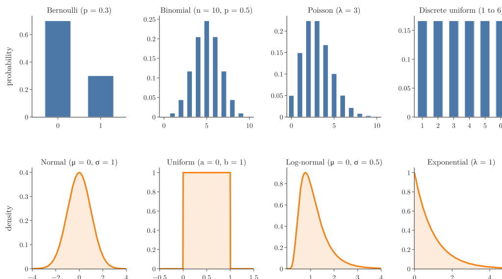
Figure 4: Eight famous distributions: four discrete (top) and four continuous (bottom), with their parameters
