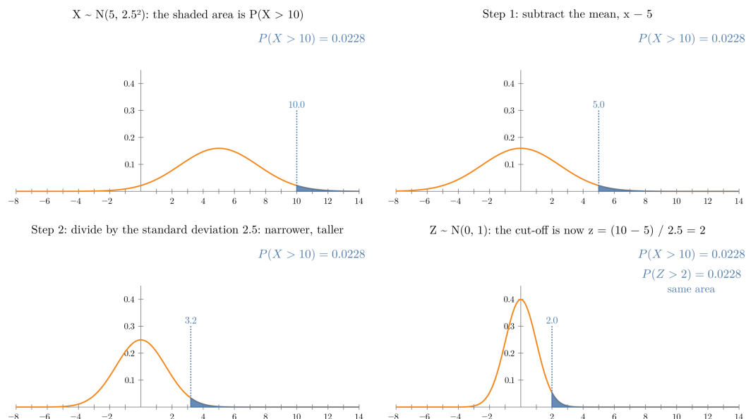
Figure 2: Standardizing as motion: X \sim N(5, 2.5^2) slides left by its mean, then squeezes by its standard deviation into N(0, 1) ; the shaded tail beyond 10, later beyond z = 2 , keeps the same area 0.0228
