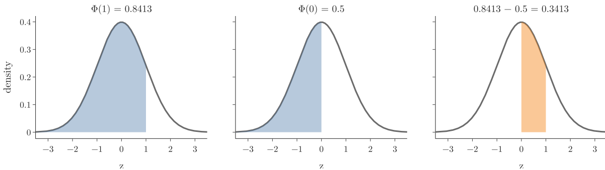
Figure 4: The area between 0 and 1 as the difference of two z-table areas
