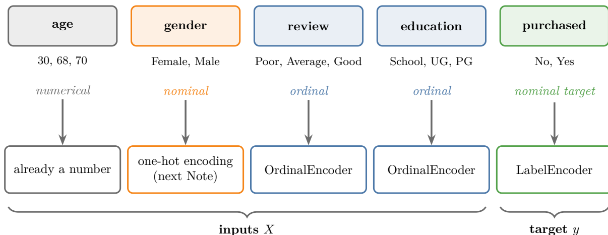
Figure 6: Each column of the customer data and the encoder it needs
