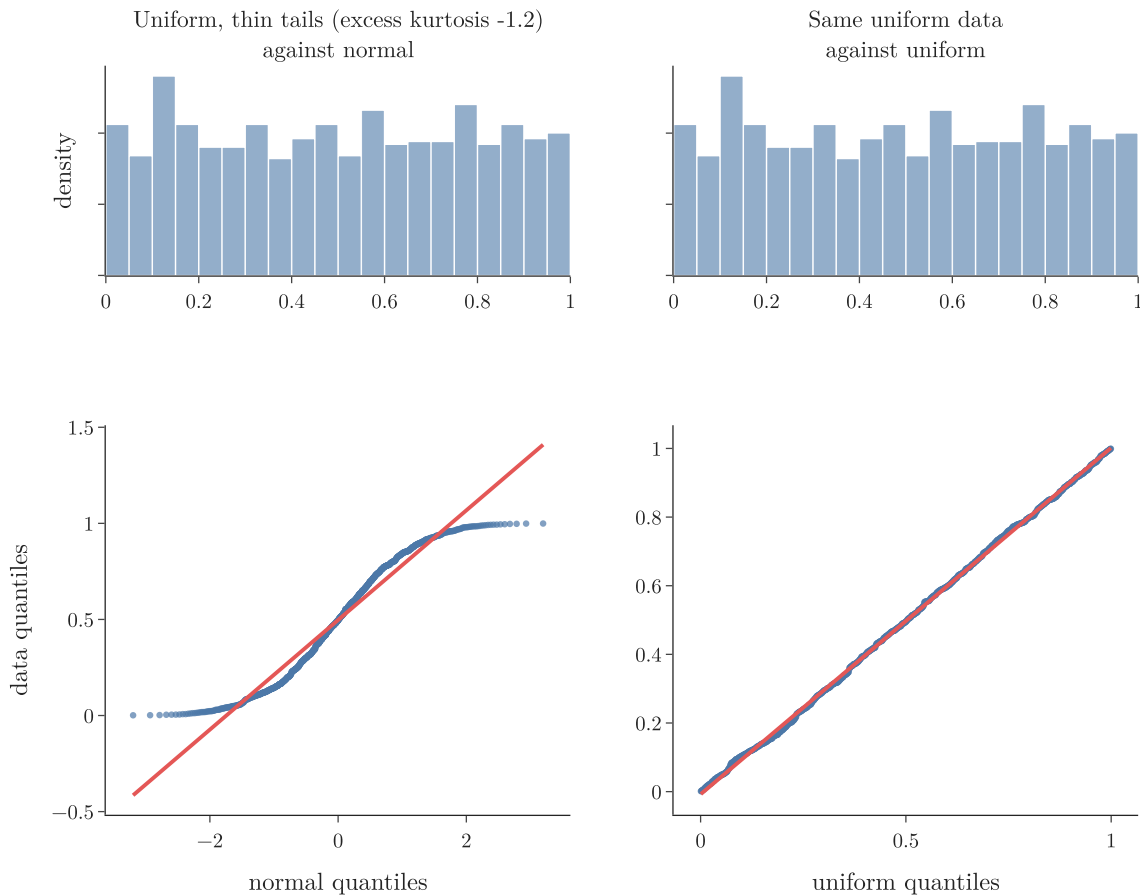
Figure 5: Top: histograms; bottom: Q-Q plots. Uniform data against the normal, then the same data against the uniform
