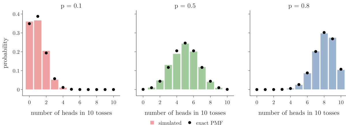
Figure 5: 1000 simulated runs of 10 tosses (bars) against the exact binomial PMF (dots)
