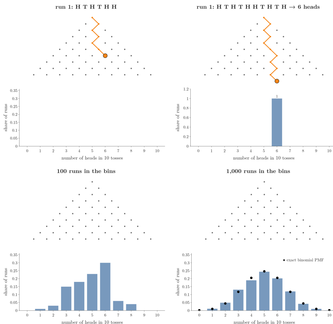
Figure 4: A Galton board for 10 fair-coin tosses: each ball is one run of 10 Bernoulli trials and lands in the bin of its head count. The bins fill with the 1000 runs above; the dots are the exact binomial PMF. Idea after Sanderson (3Blue1Brown), “But what is the Central Limit Theorem?”
