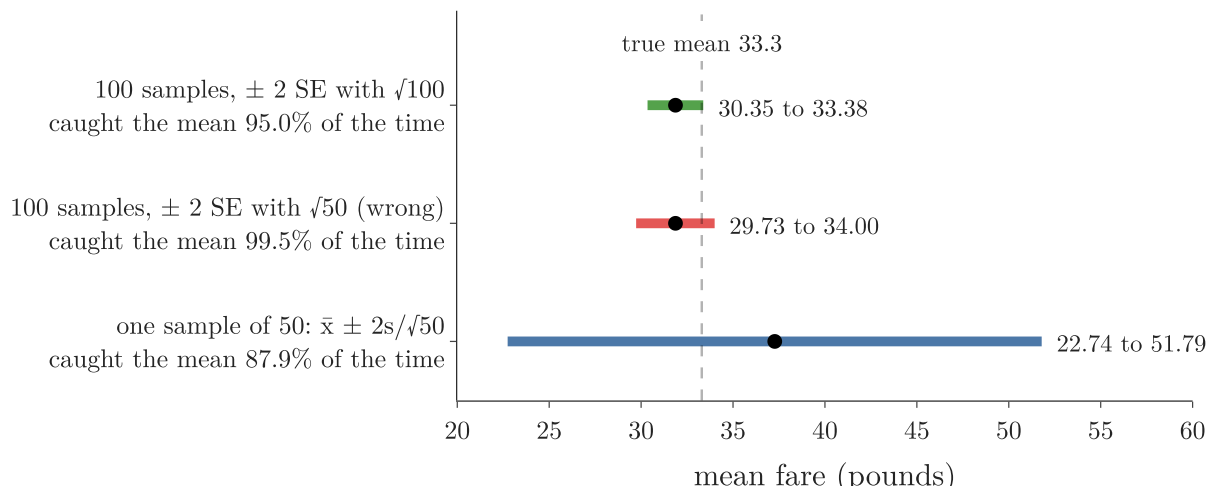
Figure 3: Three ranges for the mean fare against the true mean 33.30; each label gives how often that method caught the true mean in 1000 repetitions
