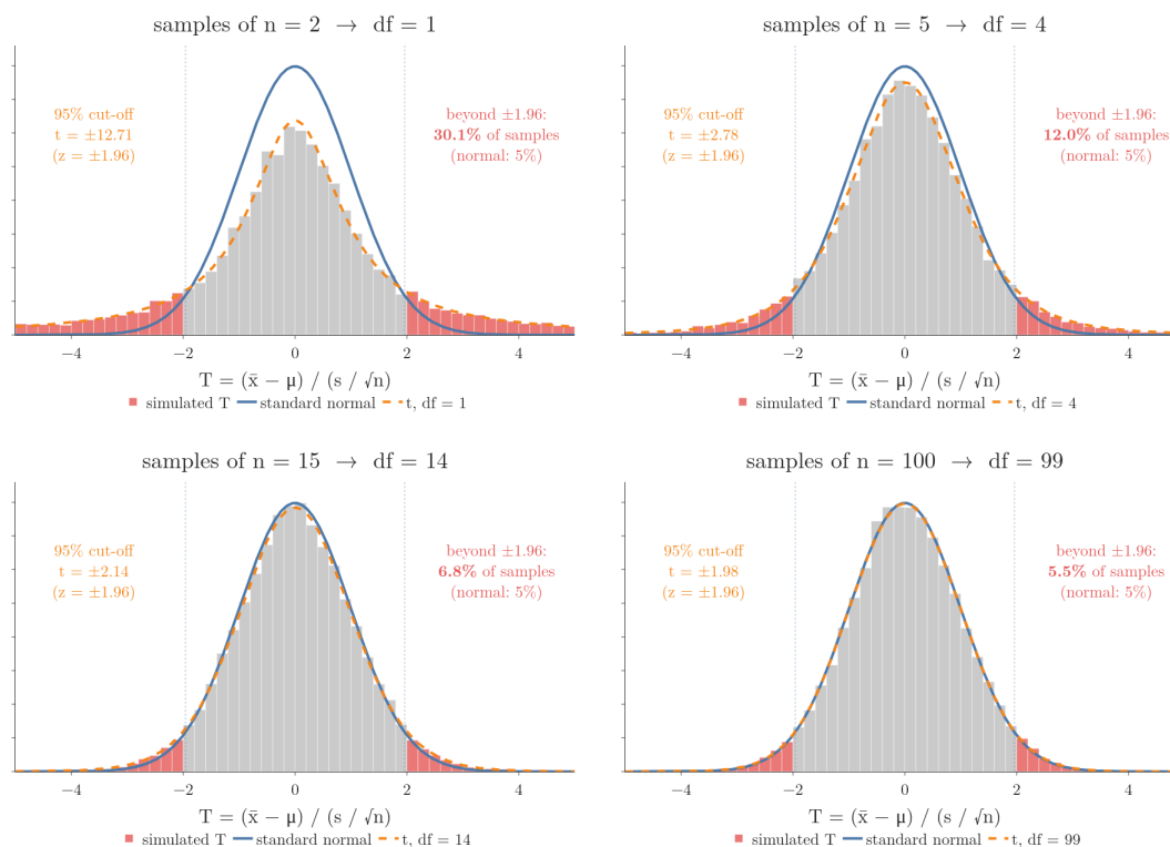
Figure 3: Simulated T values for samples of n = 2 to 100 (histogram) against the standard normal (blue) and the t-curve with df = n - 1 (orange); the share beyond \pm 1.96 falls from 30% towards 5%
