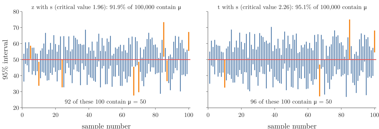
Figure 4: The same 100 samples of n = 10 with two 95% intervals each; coverage over 100,000 samples in the titles
