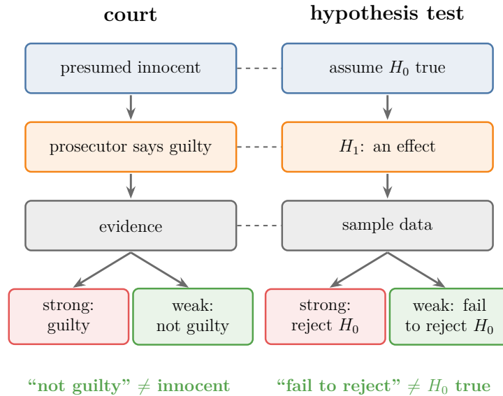
Figure 4: The courtroom and the hypothesis test, step for step. Both end in one of two verdicts, and the weak-evidence verdict proves nothing
