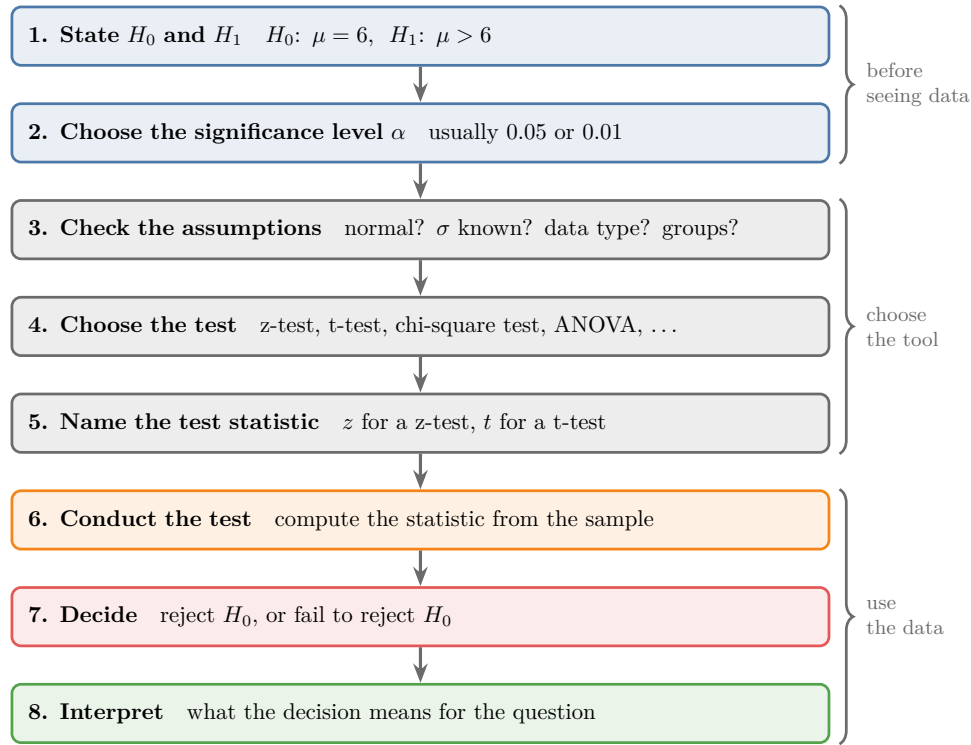
Figure 5: The eight steps of a hypothesis test (rejection region approach)
