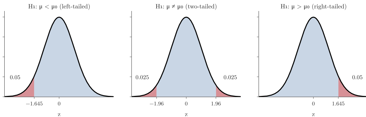
Figure 4: Rejection regions (red) at \alpha = 0.05 for the three kinds of alternative hypothesis
