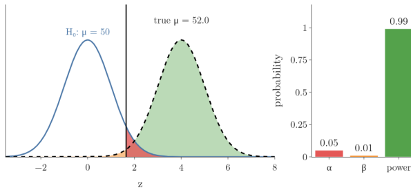
Figure 3: The three knobs of a test's power, for the training-program test. 1: \alpha from 0.10 to 0.01 ( \beta grows from 0.18 to 0.55). 2: n from 10 to 100 (power reaches 0.99). 3: the true mean from 50 to 54 (at 50 the power equals \alpha ). Red = \alpha , orange = \beta , green = power
