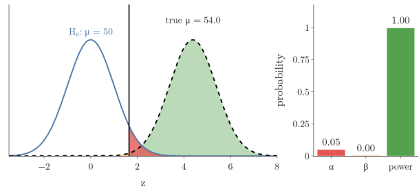
Figure 3: The three knobs of a test's power, for the training-program test. 1: \alpha from 0.10 to 0.01 ( \beta grows from 0.18 to 0.55). 2: n from 10 to 100 (power reaches 0.99). 3: the true mean from 50 to 54 (at 50 the power equals \alpha ). Red = \alpha , orange = \beta , green = power
