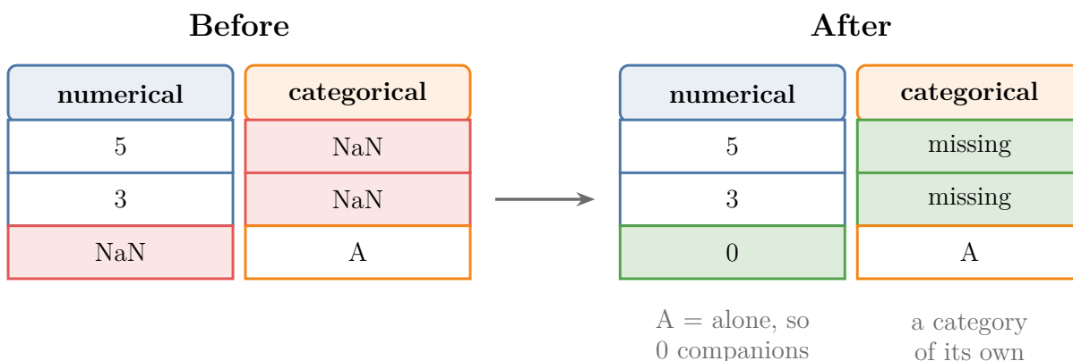
Figure 7: The gaps of the Type 2 split (rows 0, 1 and 4), before and after filling
