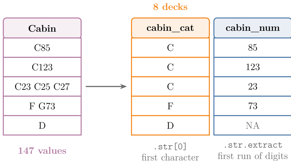
Figure 5: Splitting Cabin on the rows of the table above: the first character becomes the deck, the first run of digits the number
