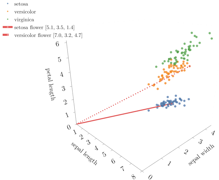
Figure 2: The iris flowers as feature vectors, using three of the four features
