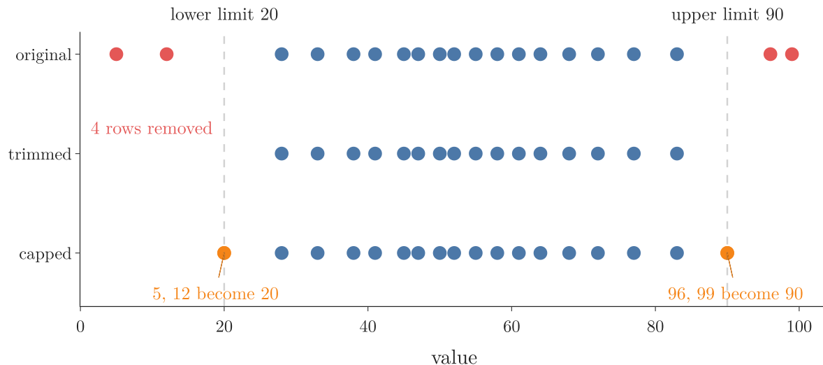
Figure 5: Trimming deletes the four outliers; capping keeps all 20 rows and moves the outliers onto the limits
