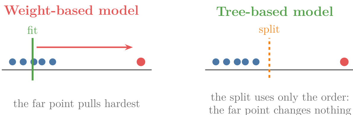
Figure 4: A weight-based fit is pulled by a far point; a tree’s split depends only on the order of the values
