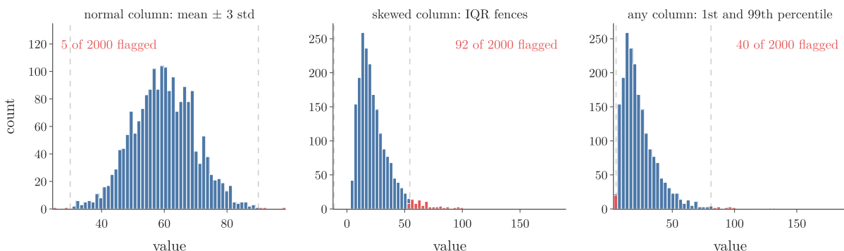
Figure 6: The three detection rules: mean plus or minus 3 standard deviations, the IQR fences, and the 1st and 99th percentiles
