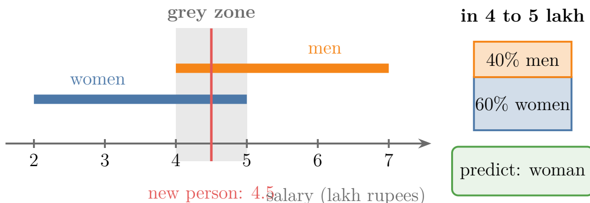
Figure 4: Salary cannot separate the two groups between 4 and 5 lakh rupees (the ranges outside that zone are drawn for illustration). With the shares 60% women and 40% men in that range, the prediction for a new person earning 4.5 lakh is “woman”
