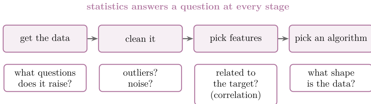
Figure 5: The questions statistics answers at each stage of an ML project
