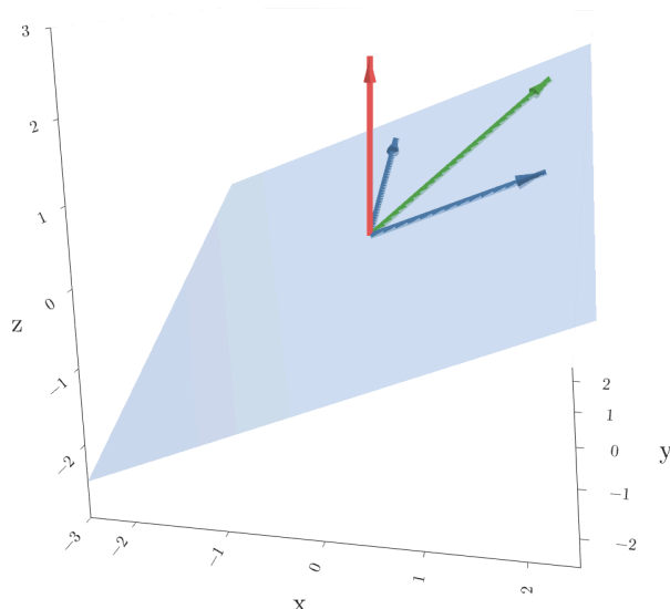
Figure 4: The plane spanned by \mathbf{v}_1 and \mathbf{v}_2 , a third vector on it (green) and one off it (red)
