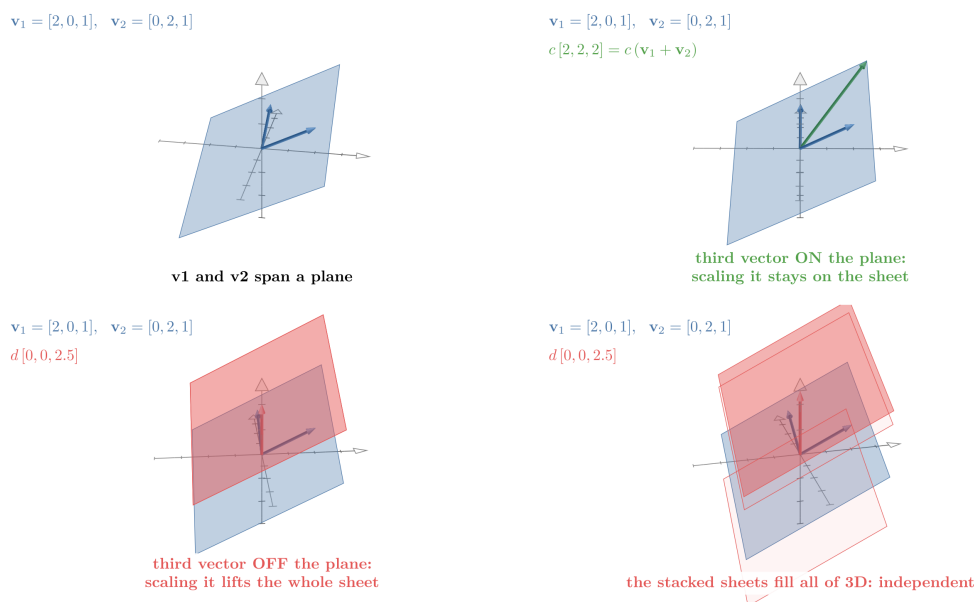
Figure 5: A third vector on the plane of \mathbf{v}_1 and \mathbf{v}_2 (green, dependent) only moves within the plane; a third vector off it (red, independent) sweeps the plane through all of space
