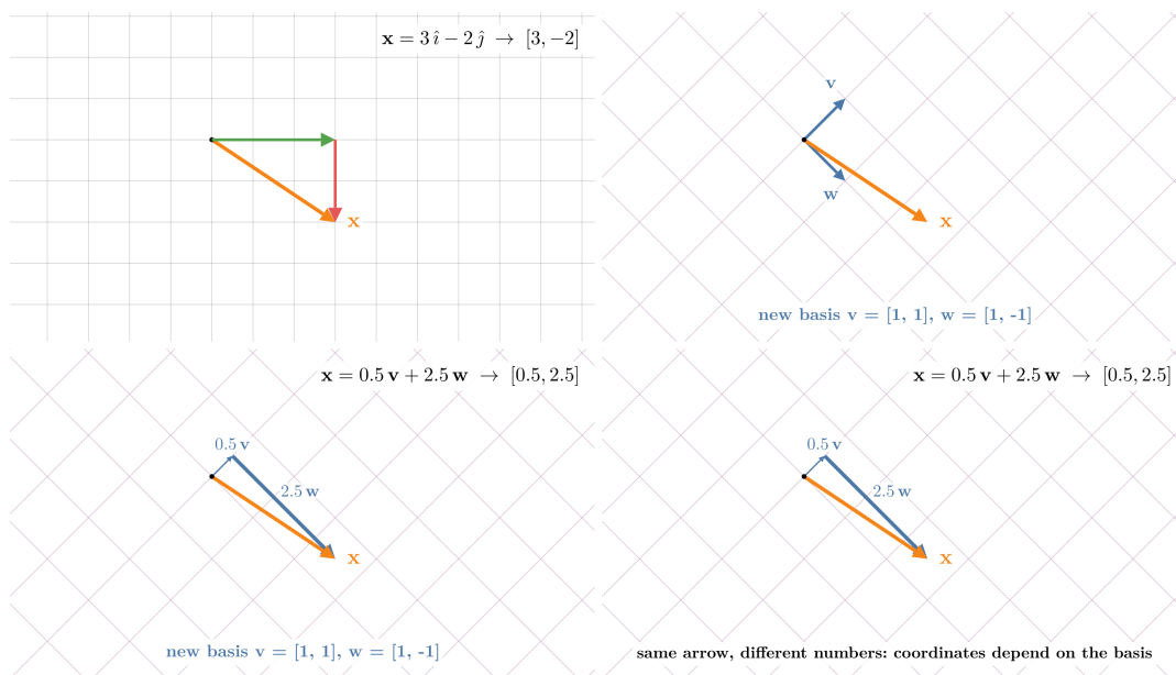
Figure 3: The arrow [3, -2] measured with two bases: 3\hat{i} - 2\hat{j} on the standard grid, and 0.5\mathbf{v} + 2.5\mathbf{w} on the grid of \mathbf{v} = [1, 1] and \mathbf{w} = [1, -1]
