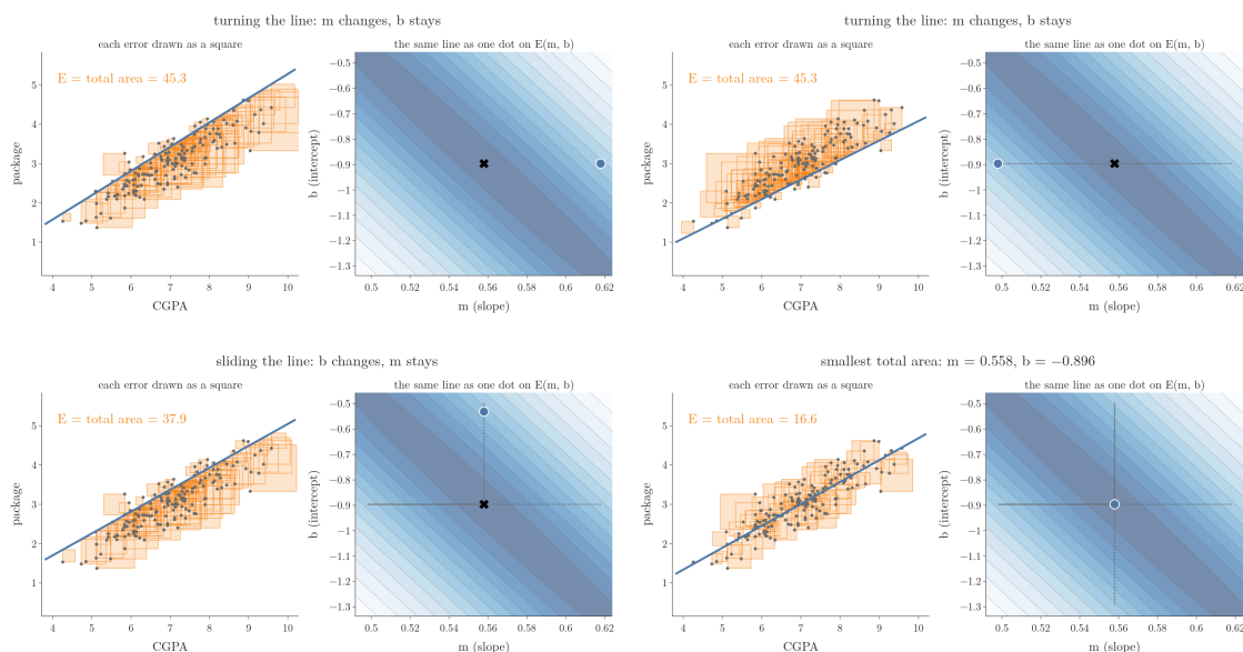
Figure 2: Turning and sliding a line through the 160 training students. Left: the squared errors as squares, with total area E . Right: the same line as a dot on the contour map of E(m, b) ; the black cross marks the smallest E .
