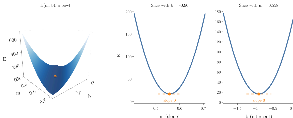
Figure 3: The error function: a bowl with the best line at the bottom
