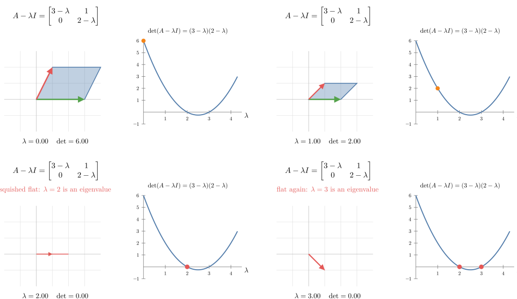
Figure 2: Turning the knob \lambda : A - \lambda I squishes the unit square flat exactly when \lambda is an eigenvalue of A
