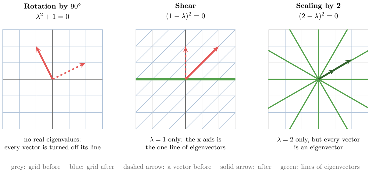
Figure 3: Three transformations with very different eigenvectors
