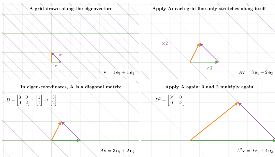
Figure 4: A grid drawn along the eigenvectors e_1 = [1, 0] and e_2 = [-1, 1] ; applying A only stretches its lines, so v = 1e_1 + 1e_2 lands on 3e_1 + 2e_2 , then 9e_1 + 4e_2
