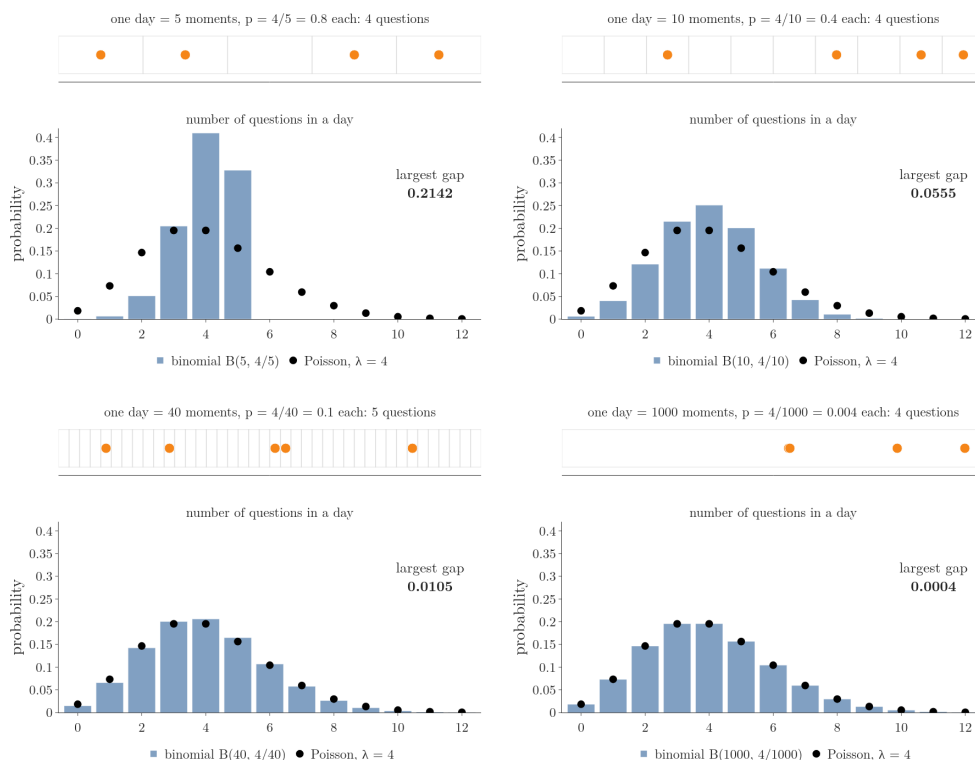
Figure 4: A day cut into n moments, each with a question with probability 4/n (top); the binomial PMF B(n, 4/n) (bars) settles onto the Poisson PMF with \lambda = 4 (dots) as n grows from 5 to 1000
