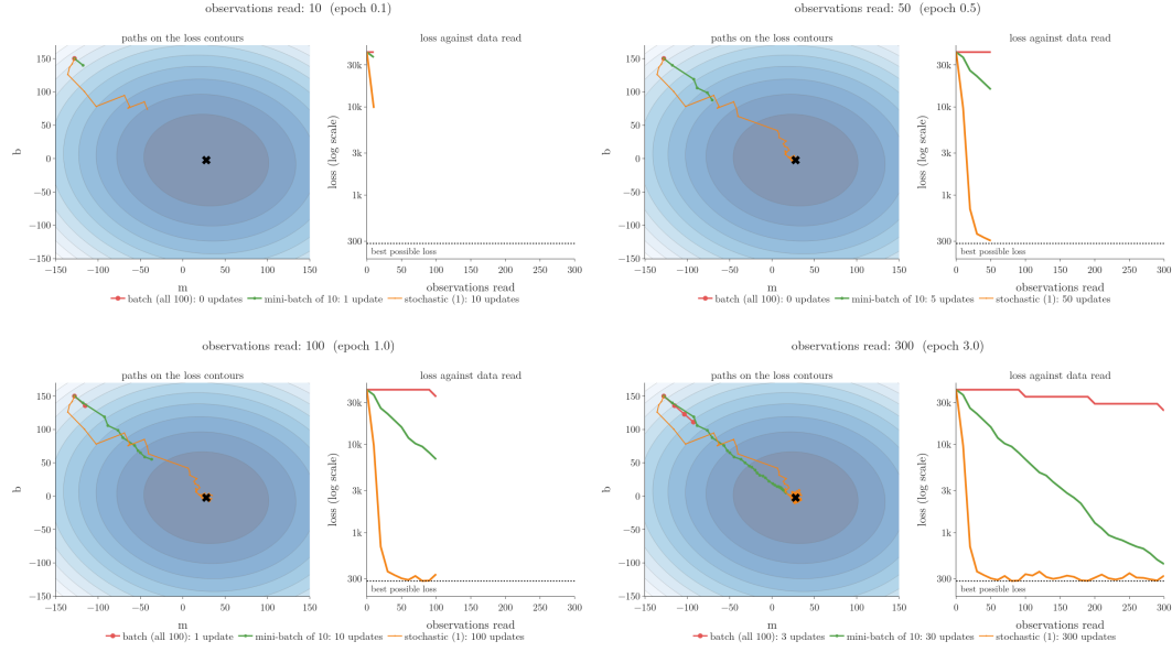
Figure 4: Batch, mini-batch and stochastic gradient descent reading the same data, 10 observations per frame, learning rate 0.05. Left: the paths on the loss contours. Right: the loss against the observations read.
