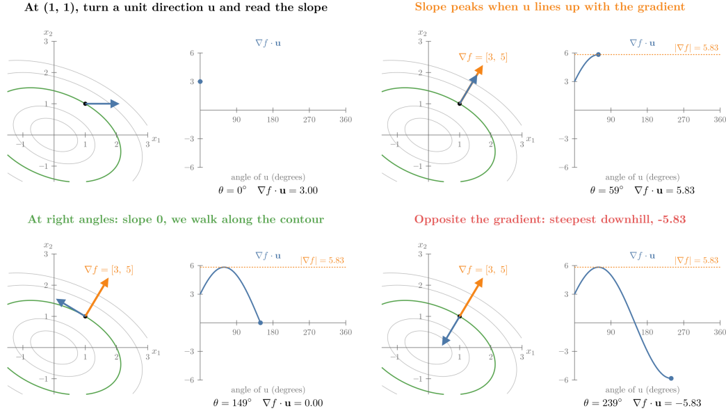
Figure 3: At (1, 1) a unit direction \mathbf{u} turns full circle (left); the slope \nabla f \cdot \mathbf{u} is traced against its angle (right): 3 along the x_1 -axis, a peak of 5.83 when \mathbf{u} lines up with \nabla f = [3, 5] , 0 along the contour line, -5.83 straight downhill
