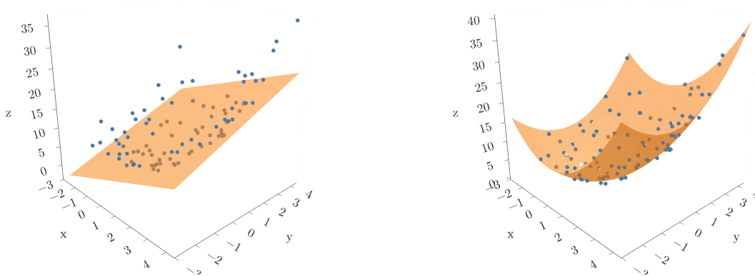
Figure 3: A plane vs a degree-2 surface on curved 3D data
