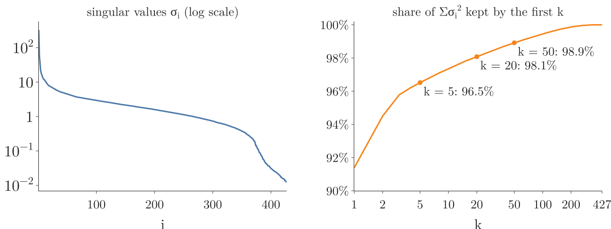
Figure 4: Singular values of the photo, and the share of \sum \sigma_i^2 kept by the first k
