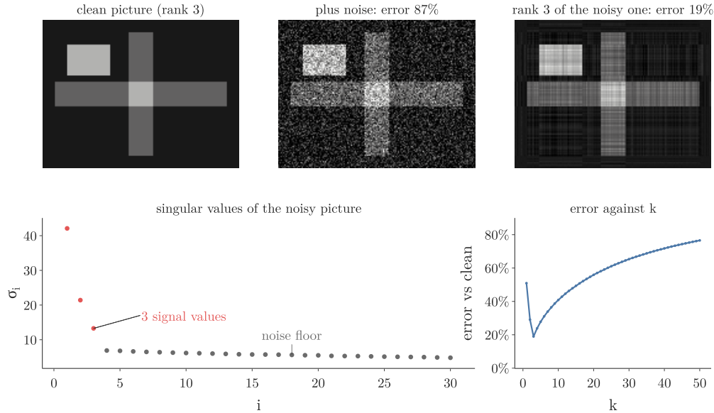
Figure 5: Noise reduction: a rank-3 picture, the same with noise, and the rank-3 approximation of the noisy one
