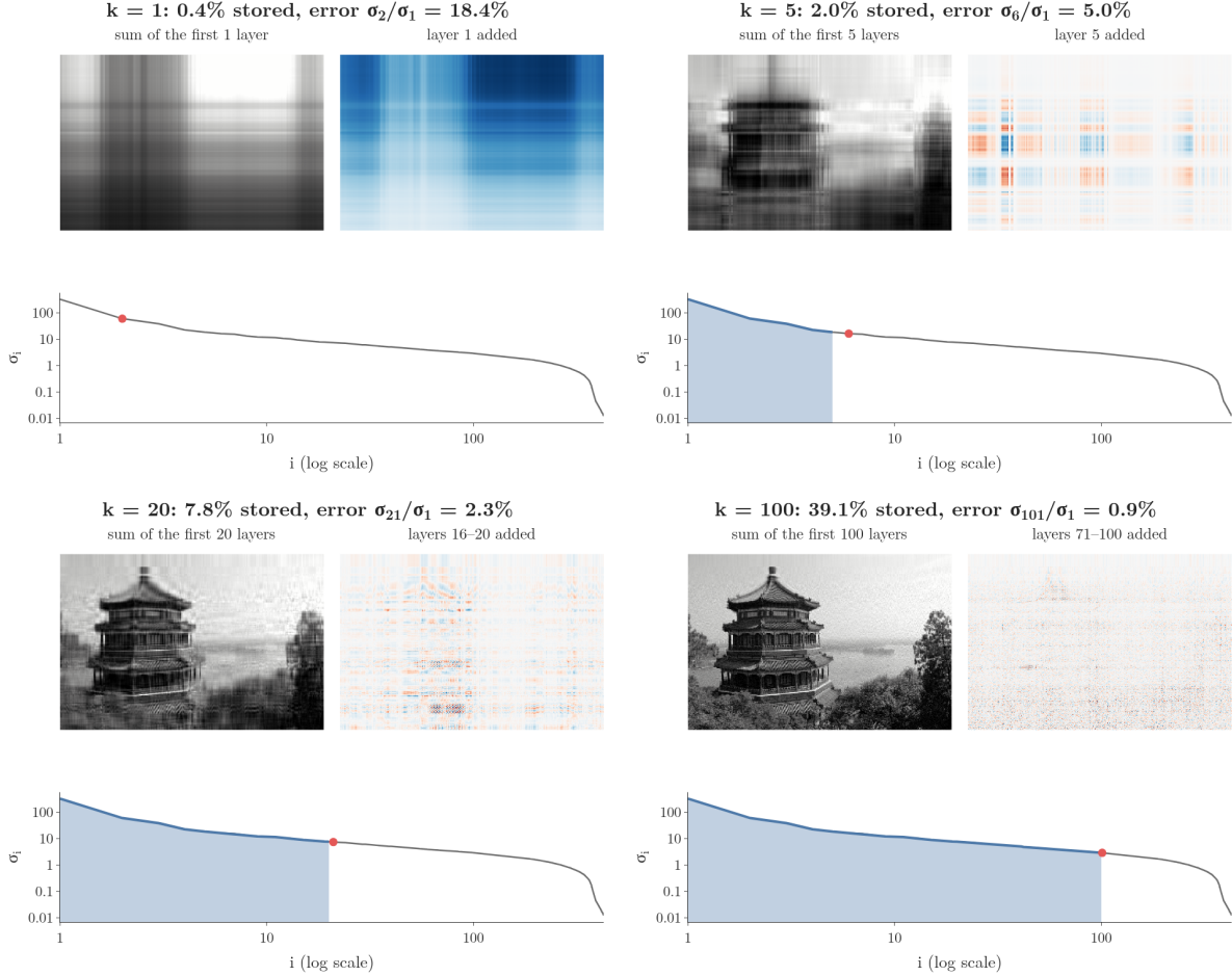
Figure 3: The photo rebuilt layer by layer, k = 1 to 100: the sum of the first k layers (left), the layers just added (right, blue positive, red negative) and the singular values kept so far (filled)
