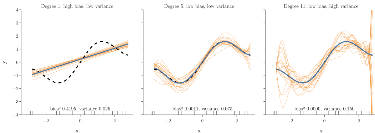
Figure 2: The same model trained on 20 different training sets. The grey ticks mark the 20 inputs shared by every training set.
