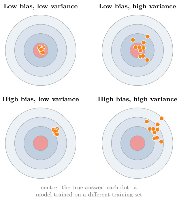
Figure 3: Bias and variance as a dartboard
