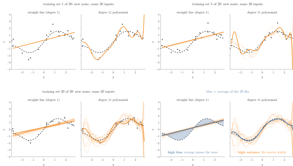
Figure 1: A straight line and a degree-11 polynomial refitted on 20 training sets (same 20 inputs, new noise each time). At the end, the blue average of the 20 fits shows the bias; the spread of the ghosts shows the variance.
