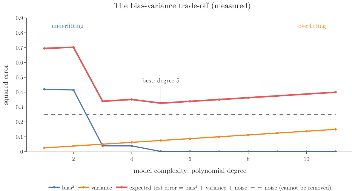
Figure 4: Bias 2 , variance and expected test error against the degree
