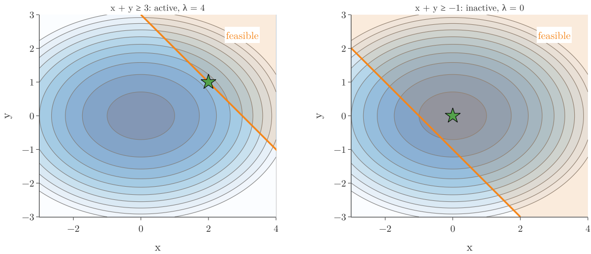
Figure 3: Minimising x^2 + 2y^2 with one inequality constraint; the feasible region is shaded and the star is the answer. Left: x + y \geq 3 cuts off the unconstrained minimum, so the answer lies on the boundary (active, \lambda = 4 ). Right: x + y \geq -1 already contains the unconstrained minimum (inactive, \lambda = 0 )
