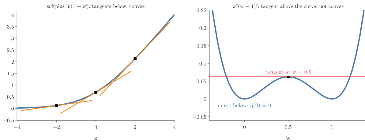
Figure 3: The first-order test. Left: every tangent of softplus lies below the curve, so it is convex. Right: the tangent of w^2(w - 1)^2 at w = 0.5 lies above the curve near 0 and 1, so it is not convex
