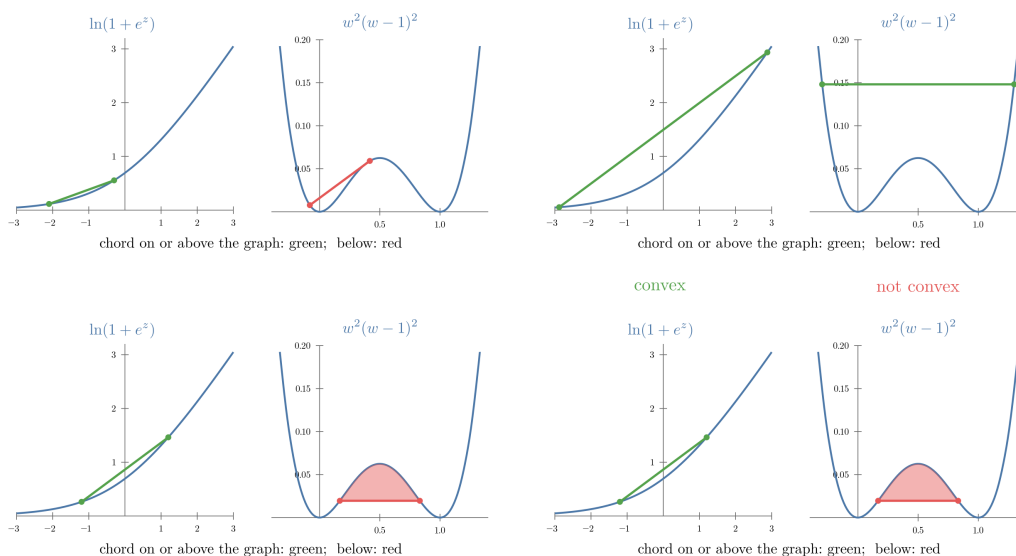
Figure 2: The chord test. A chord joins two points of each graph and slides. Left: softplus, every chord stays on or above the graph (green). Right: w^2(w-1)^2 , the chord from w = 0.17 to 0.83 runs below the hump (red gap), so the function is not convex
